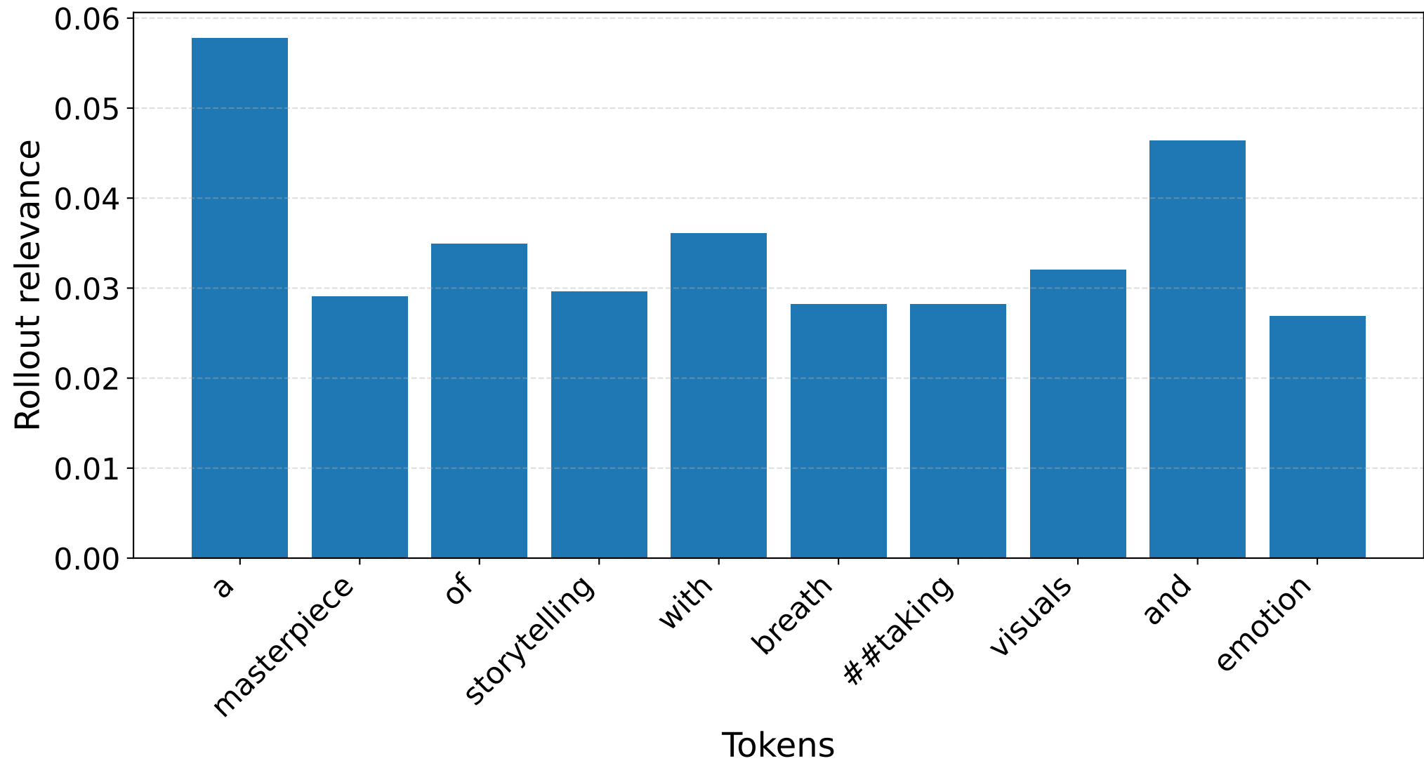
S6 [POS] — Standard rollout CLS row (filtered tokens)
