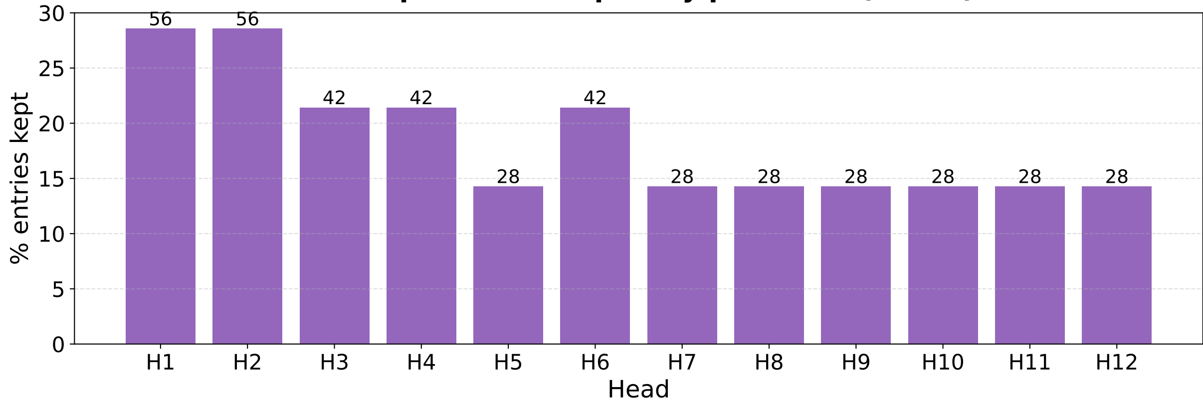
S7 Step 2 — Mask sparsity per head (K=0.0)
