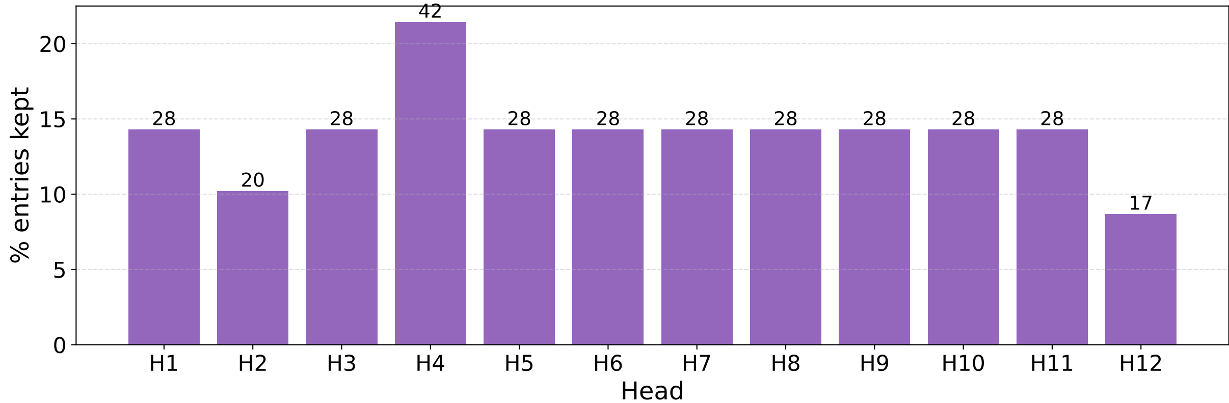
S7 Step 2 — Mask sparsity per head (K=0.5)
