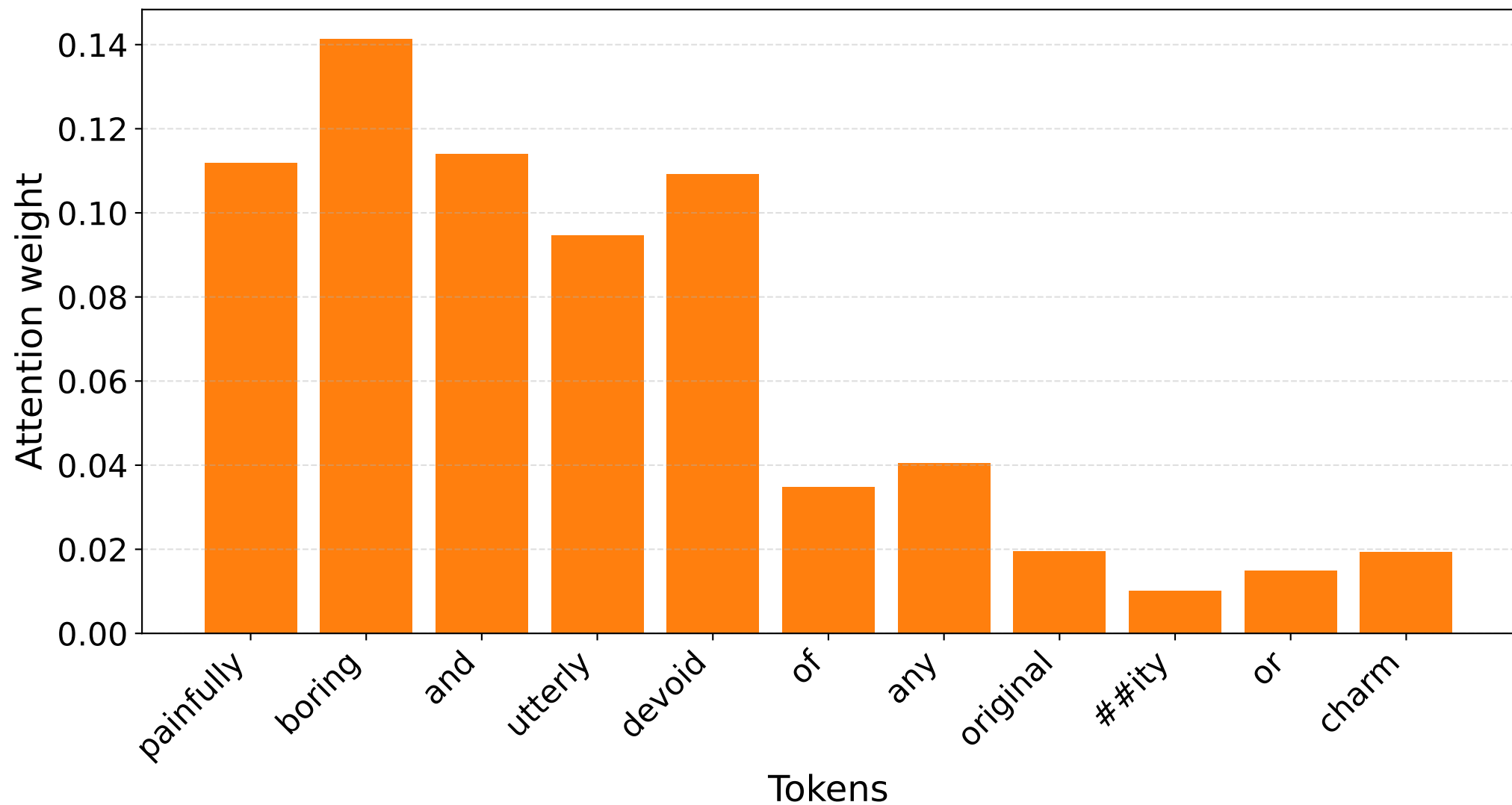
S7 [NEG] — Raw attention CLS row (filtered tokens)
