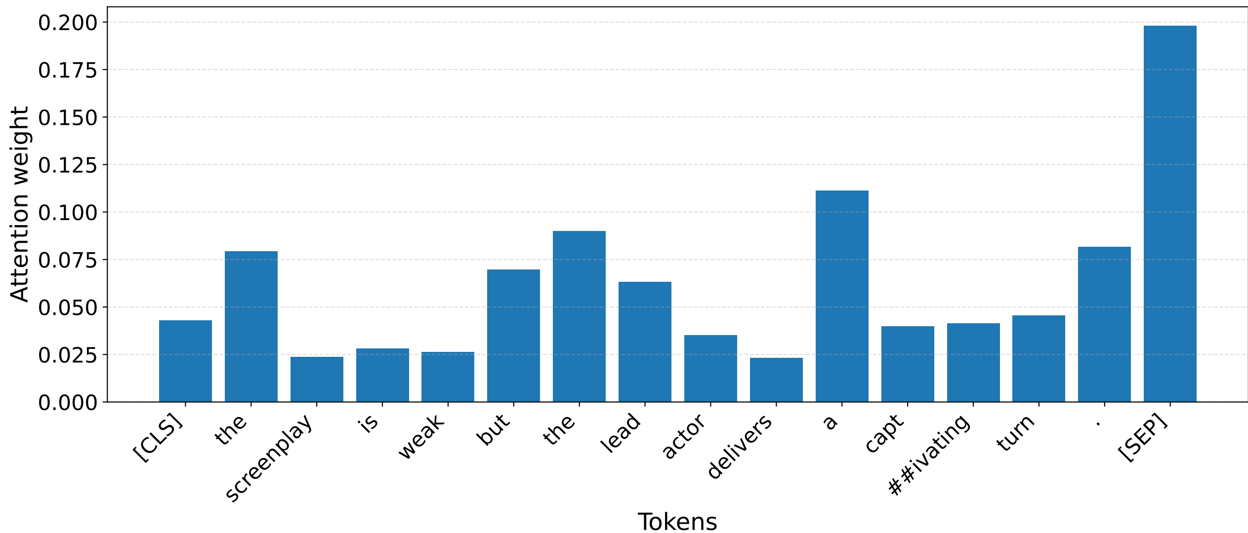
S8 [POS] — Vanilla attention CLS row (Layer 1, Head 1)
