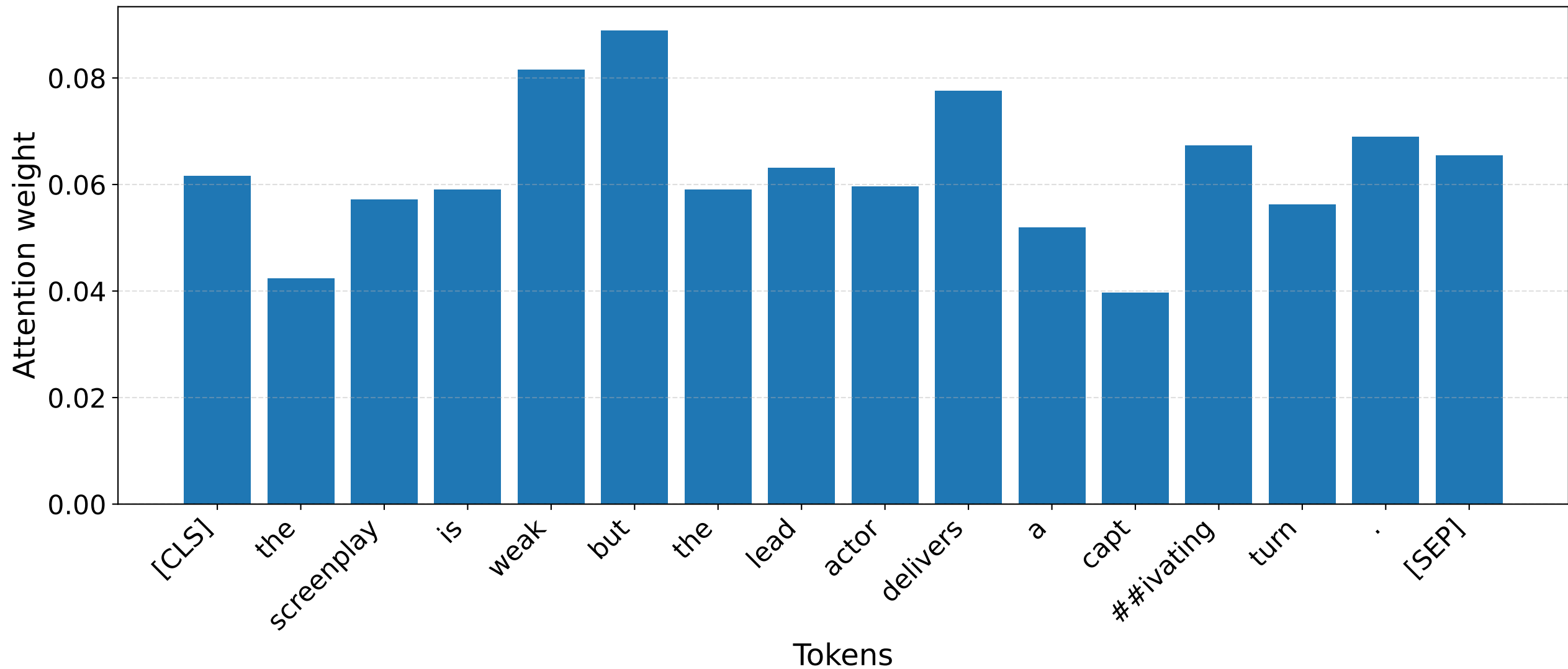
S8 [POS] — Vanilla attention CLS row
