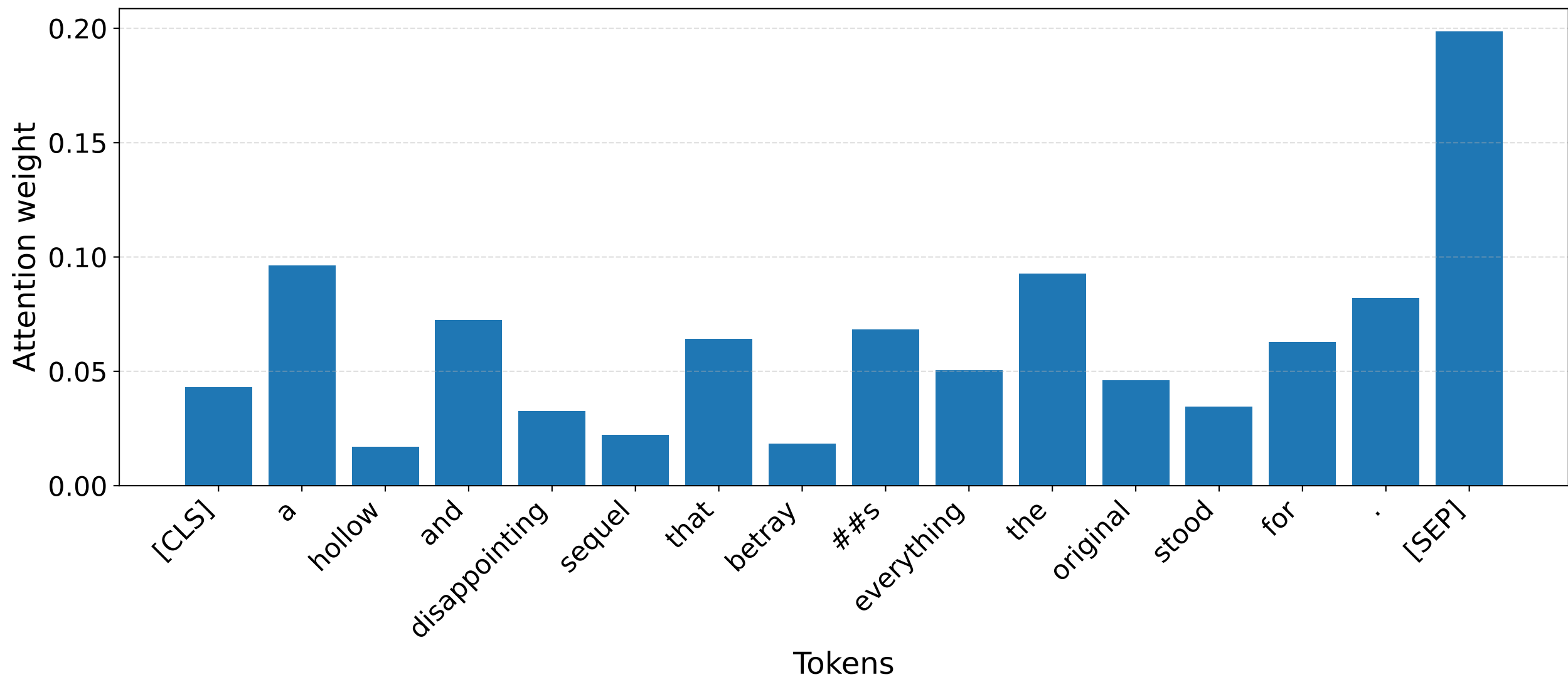
S9 [NEG] — Vanilla attention CLS row (Layer 1, Head 1)
