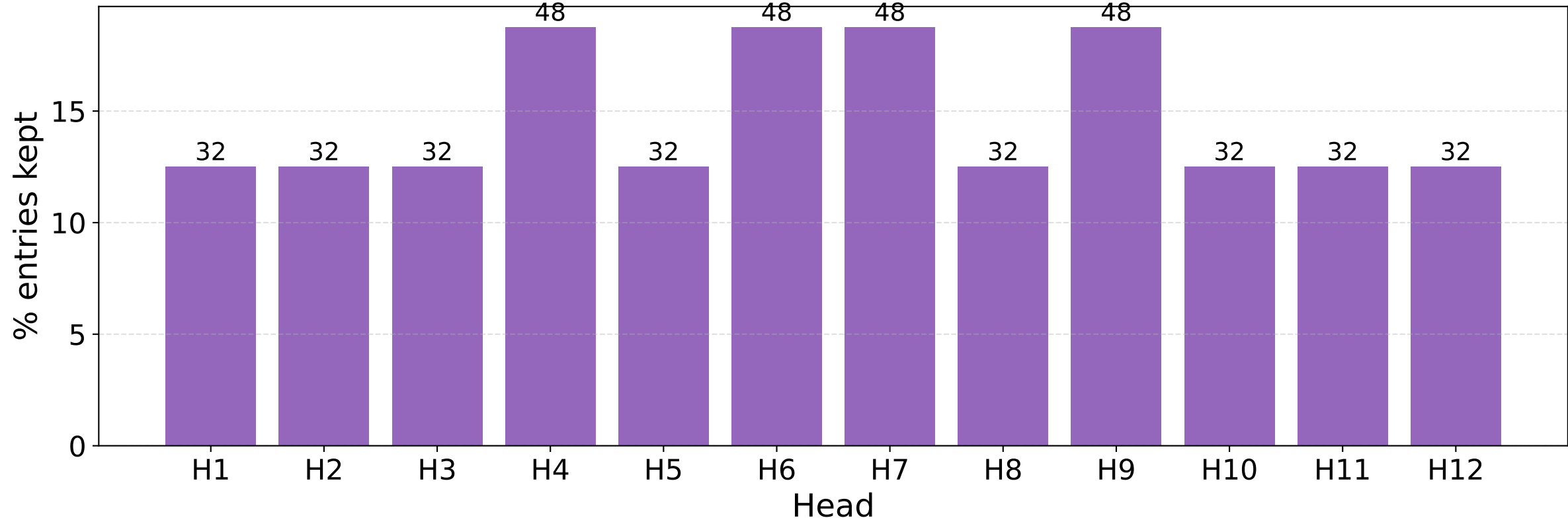
S9 Step 2 — Mask sparsity per head (K=0.5)
