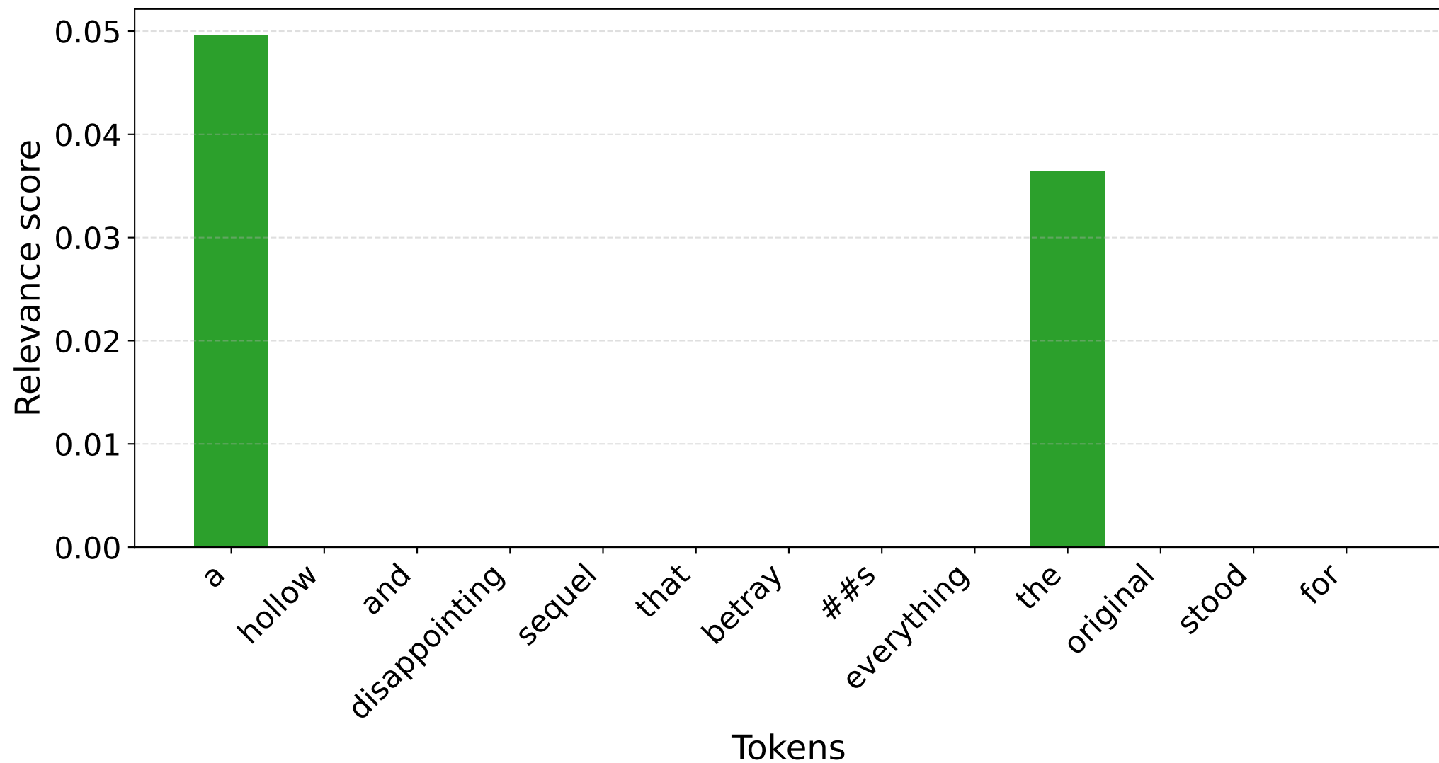
S9 [NEG] — Modified RFEM CLS row (K=0.3)
