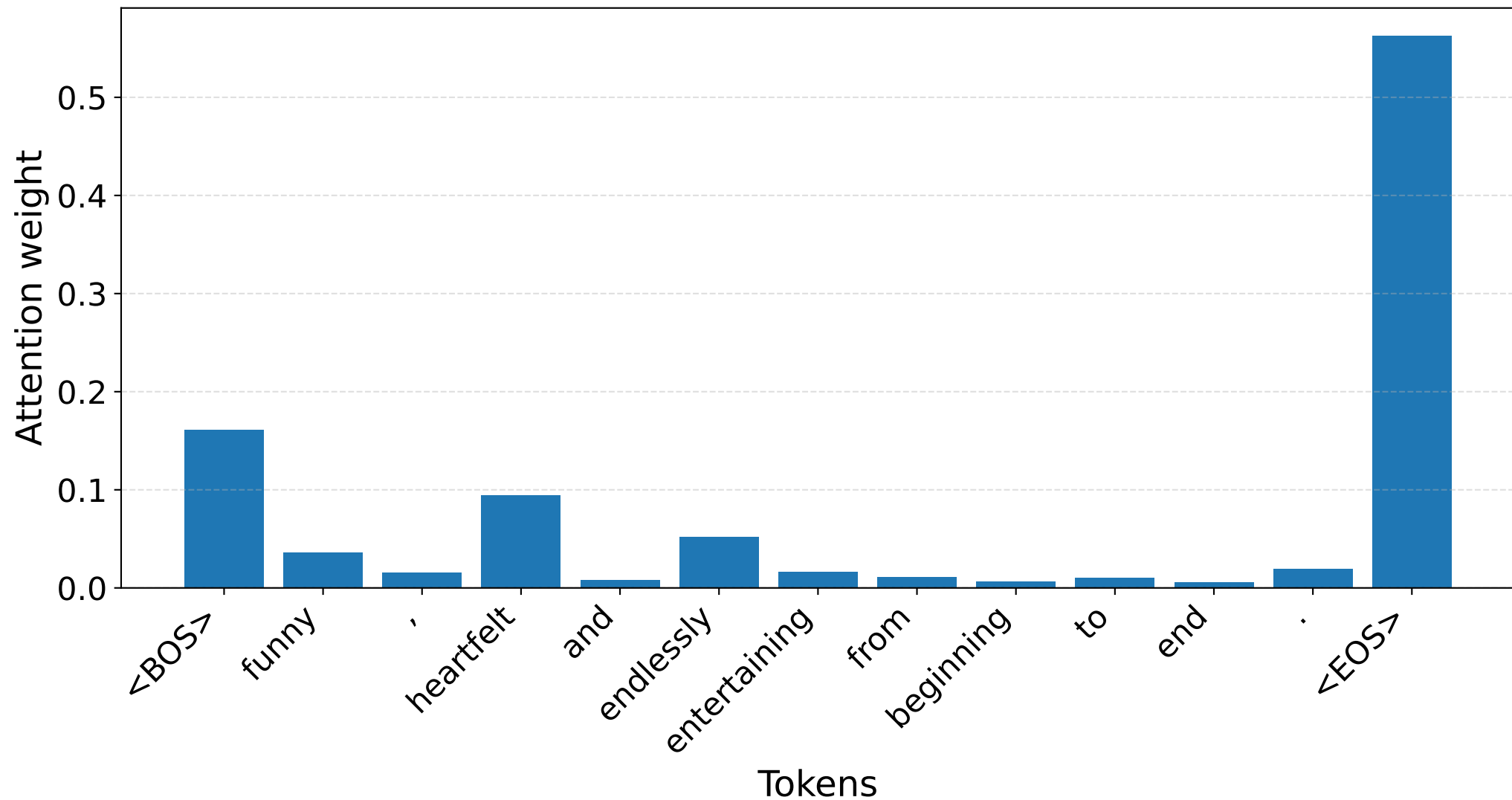
S10 [POS] — Vanilla attention EOS row (Layer 1, Head 1)
