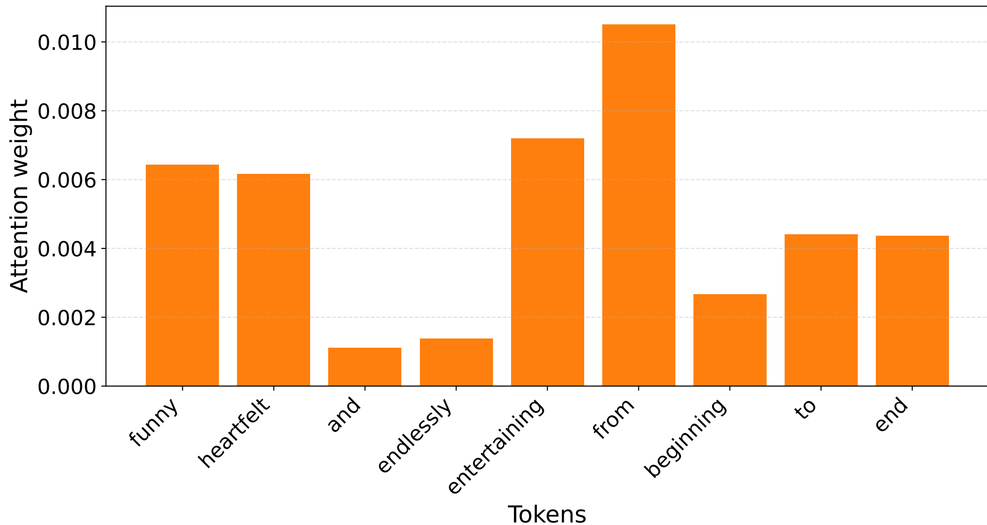
S10 [POS] — Raw attention EOS row (filtered tokens)
