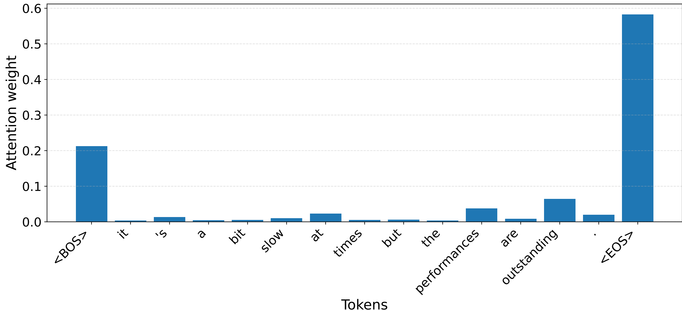
S3 [POS] — Vanilla attention EOS row (Layer 1, Head 1)
