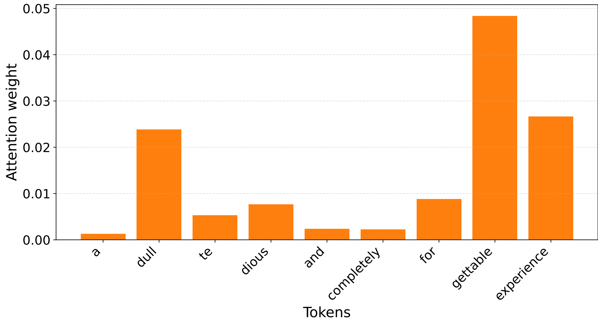
S4 [NEG] — Raw attention EOS row (filtered tokens)
