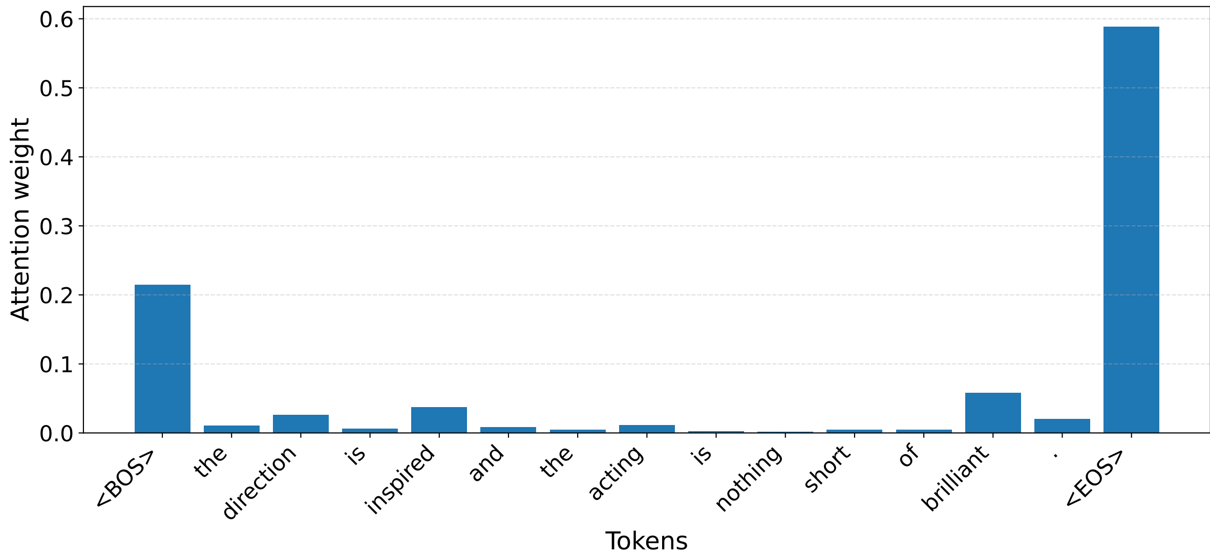
S5 [POS] — Vanilla attention EOS row (Layer 1, Head 1)
