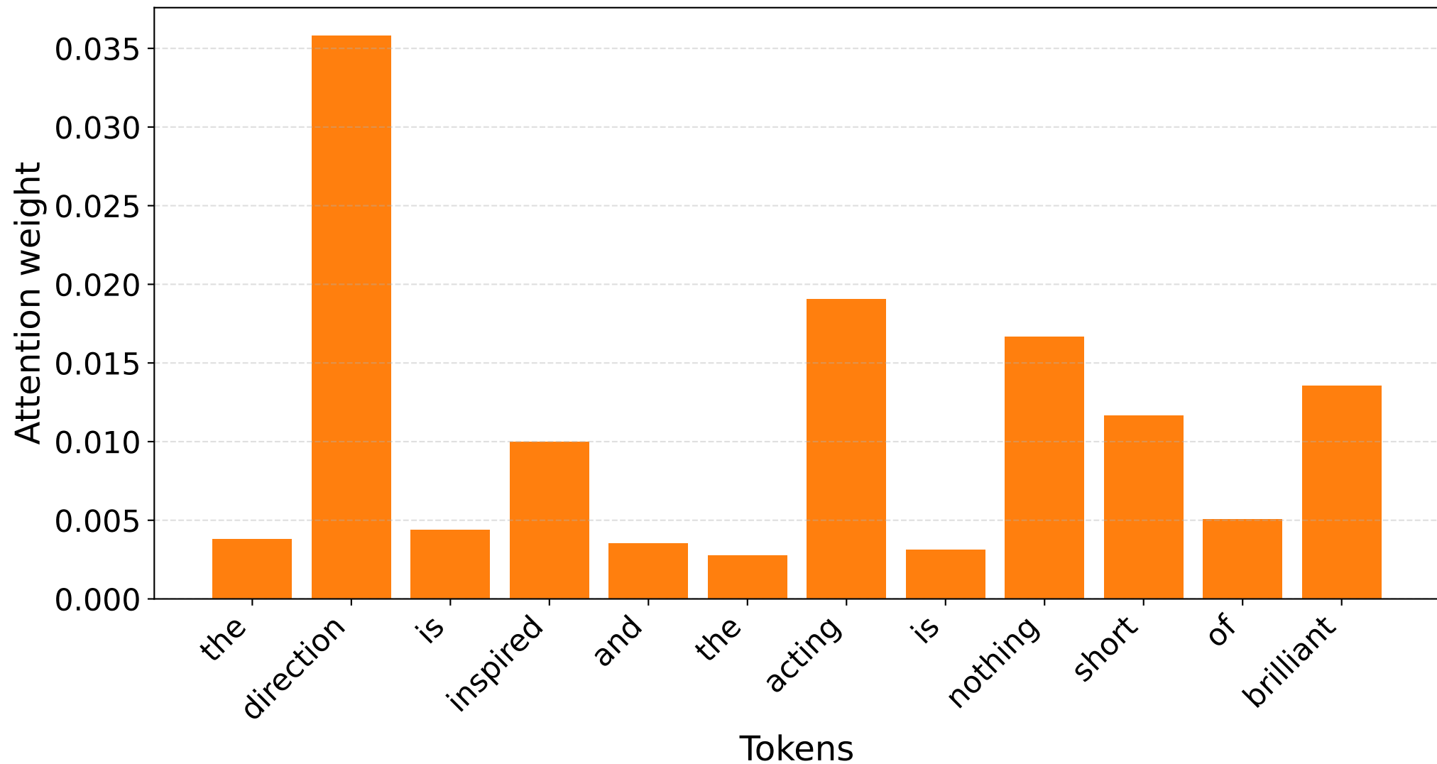
S5 [POS] — Raw attention EOS row (filtered tokens)
