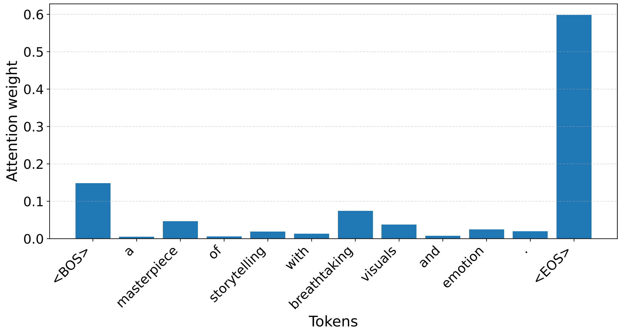
S6 [POS] — Vanilla attention EOS row (Layer 1, Head 1)
