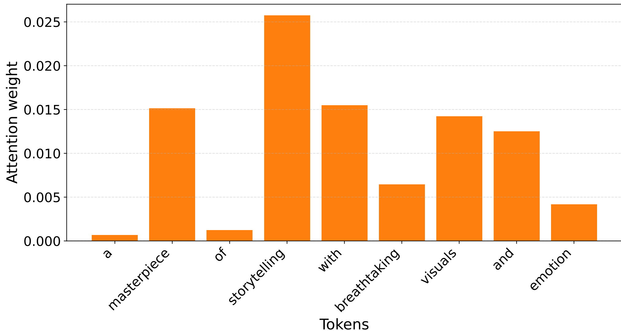
S6 [POS] — Raw attention EOS row (filtered tokens)
