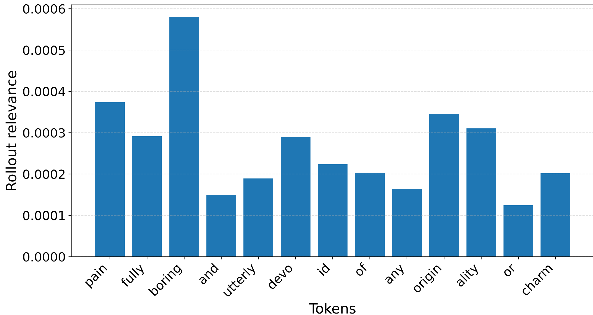
S7 [NEG] — Standard rollout EOS row (filtered tokens)
