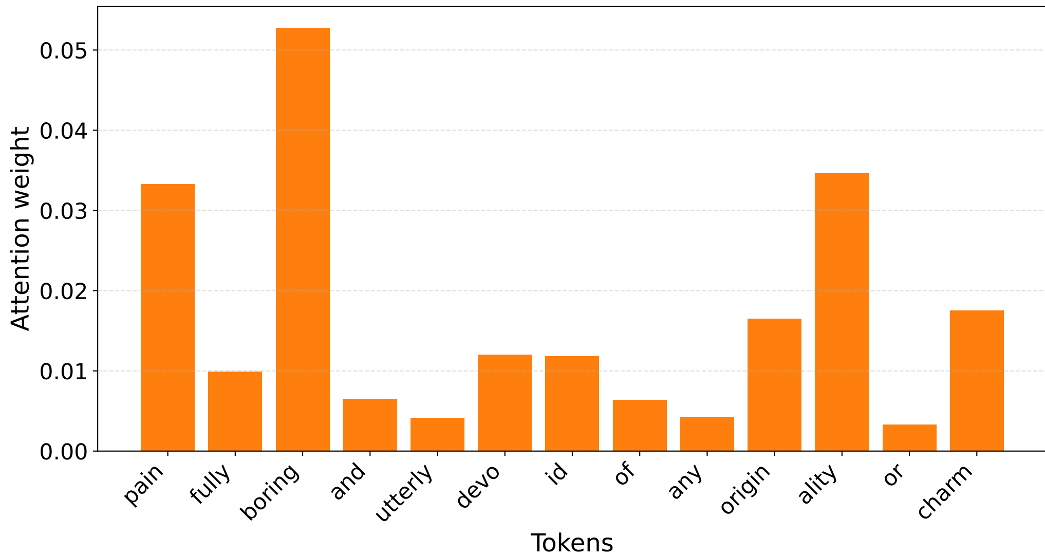
S7 [NEG] — Raw attention EOS row (filtered tokens)
