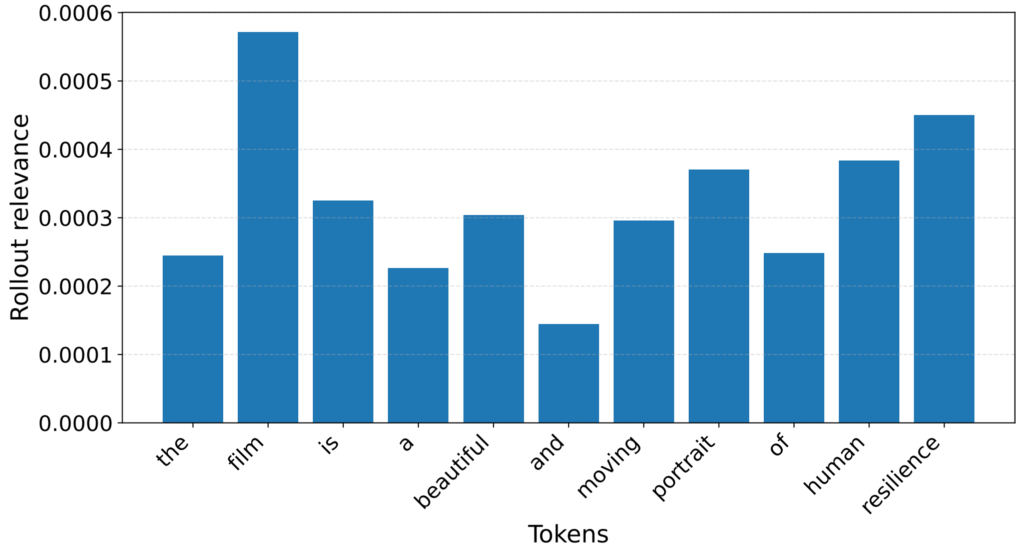
S1 [POS] — Standard rollout EOS row (filtered tokens)
