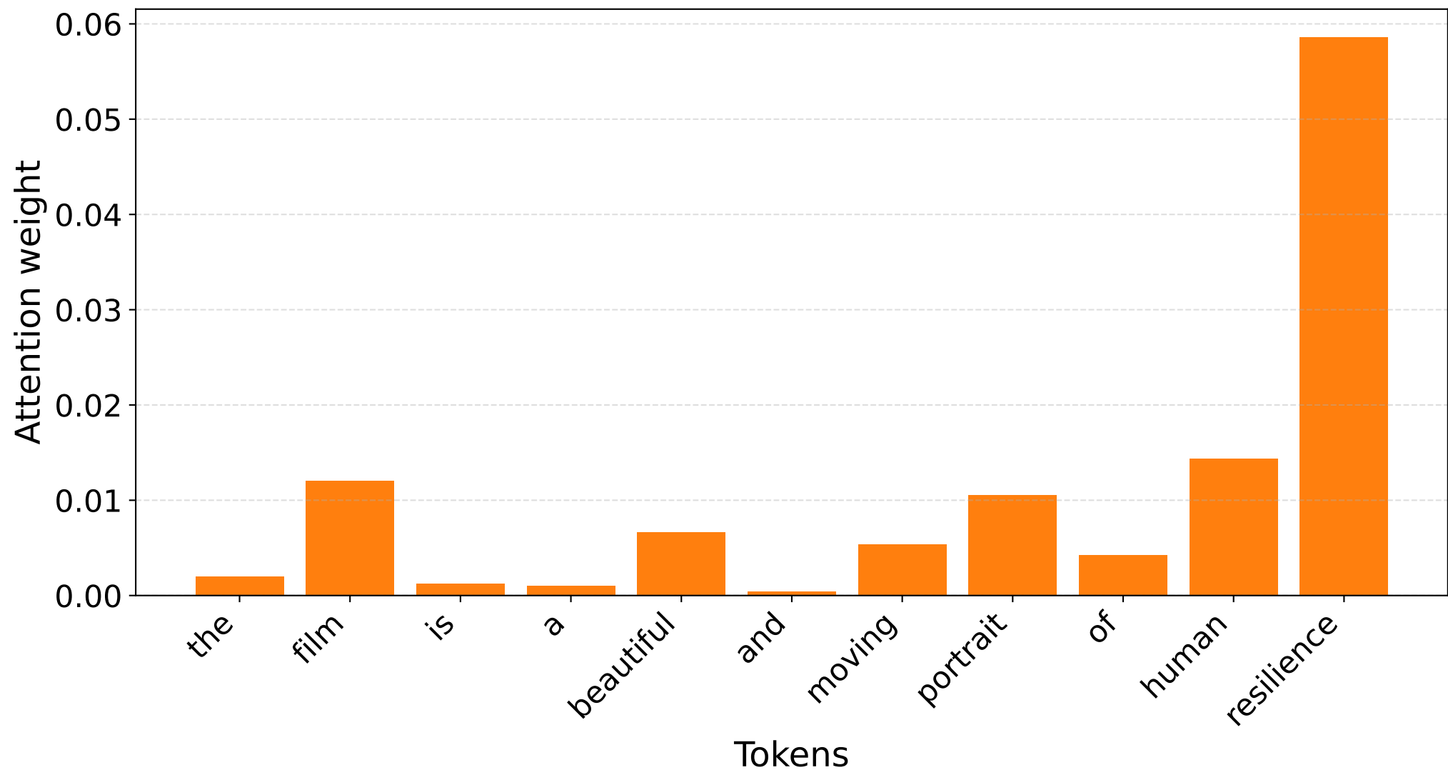
S1 [POS] — Raw attention EOS row (filtered tokens)
