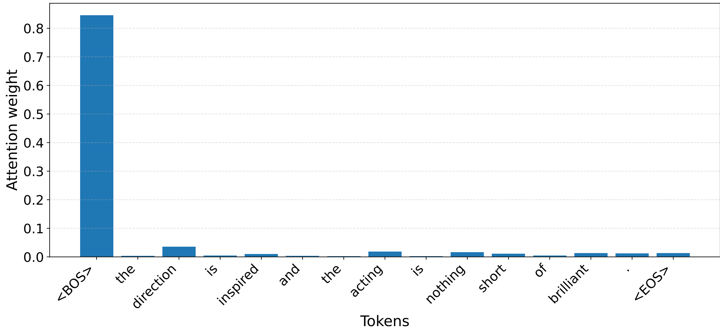
S5 [POS] — Vanilla attention EOS row
