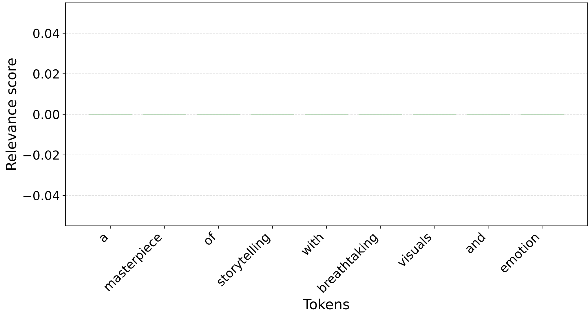
S6 [POS] — Modified RFEM EOS row (K=0.3)
