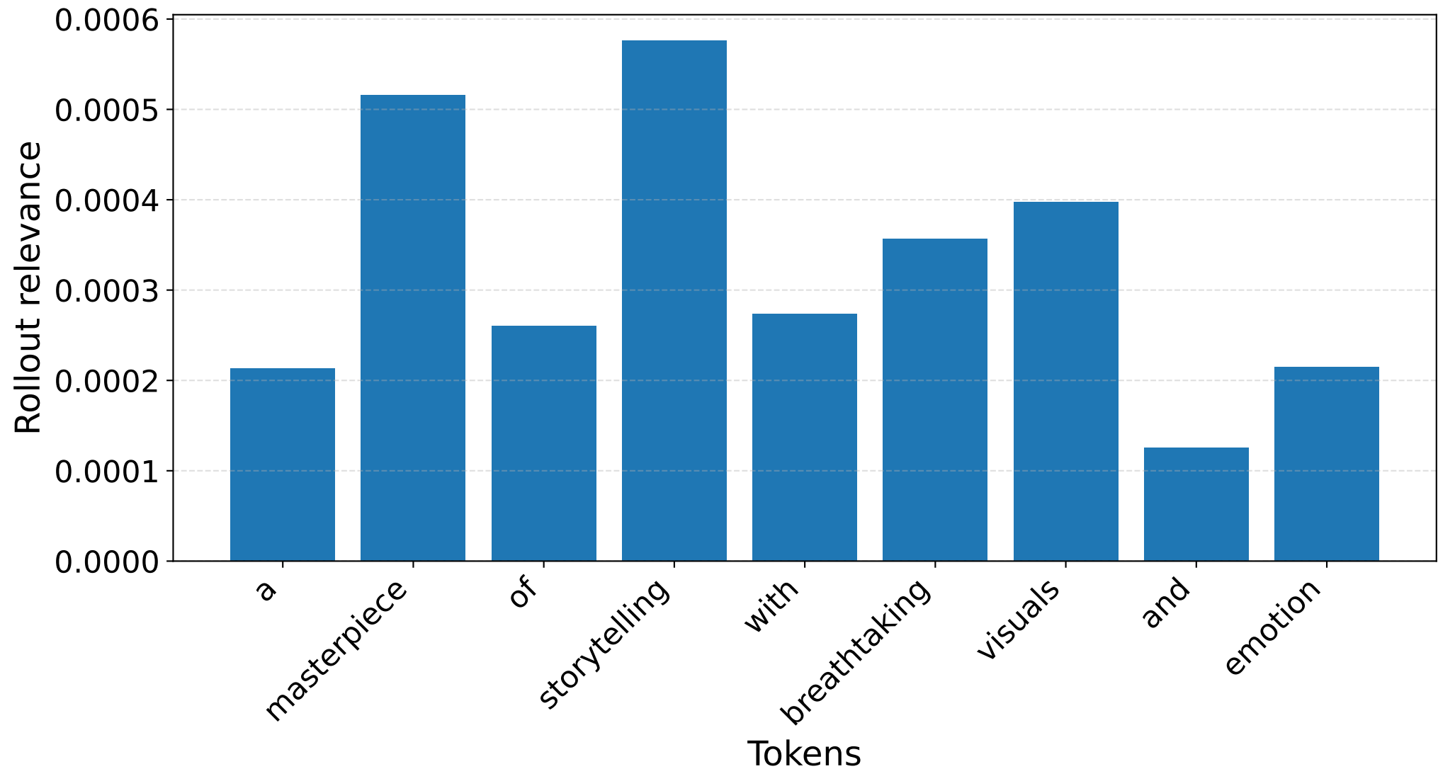
S6 [POS] — Standard rollout EOS row (filtered tokens)
