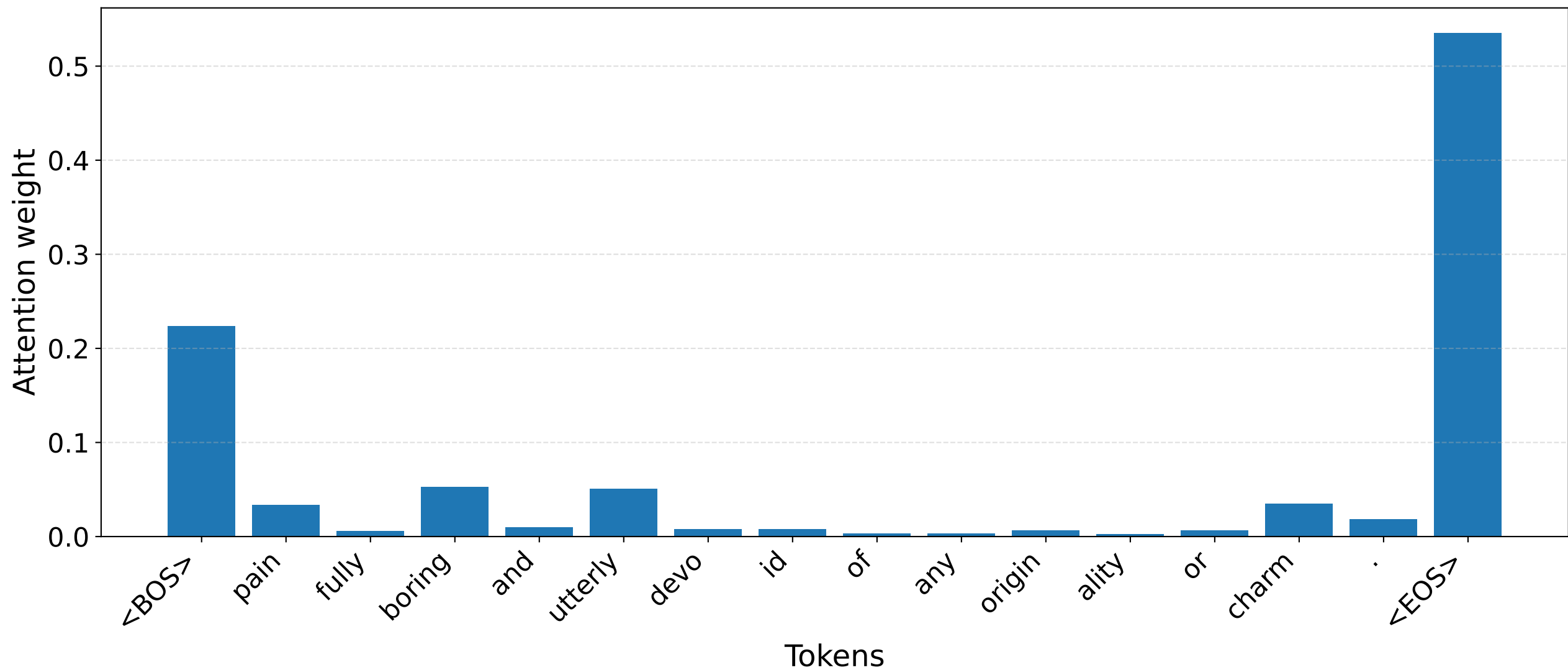
S7 [NEG] — Vanilla attention EOS row (Layer 1, Head 1)
