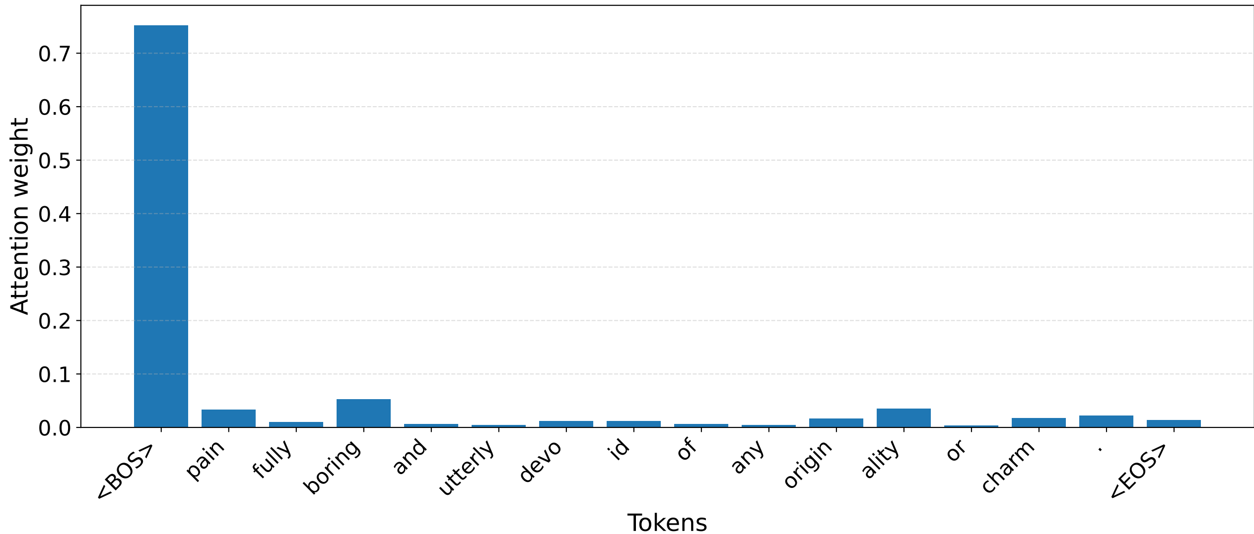
S7 [NEG] — Vanilla attention EOS row
