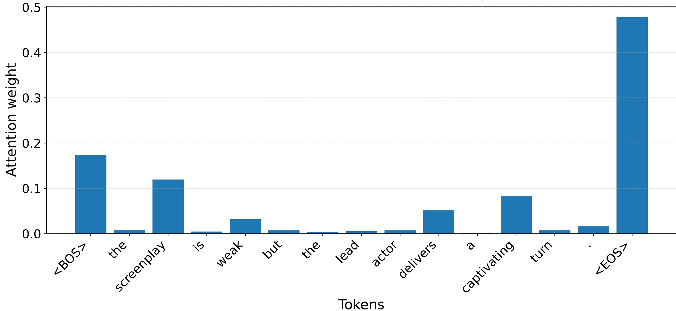
S8 [POS] — Vanilla attention EOS row (Layer 1, Head 1)
