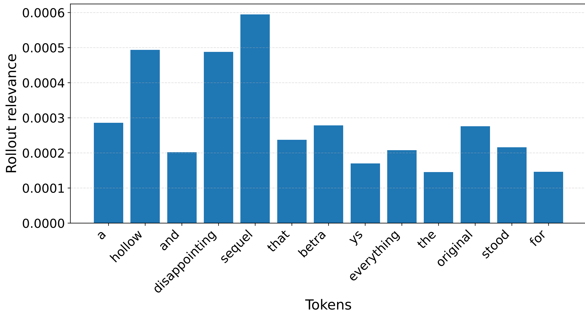
S9 [NEG] — Standard rollout EOS row (filtered tokens)
