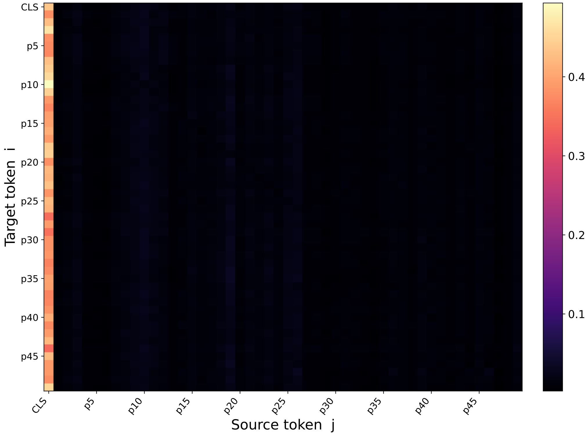
10815824_2997e03d76 [vanilla] — Layer 1, Head 1 attention matrix \mu = 0.02000 \sigma = 0.054862
