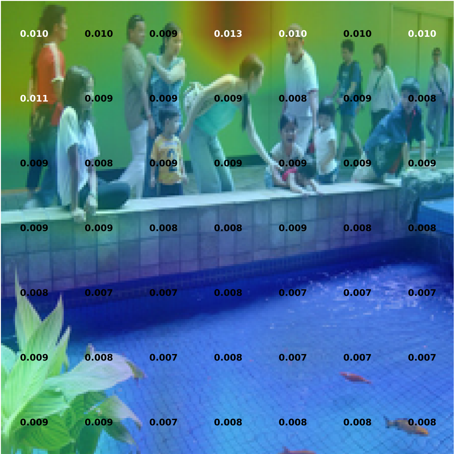
12830823_87d2654e31 [rollout] — Standard rollout CLS overlay (values) \mu = 0.00856 \sigma = 0.001104 (49 patches)
