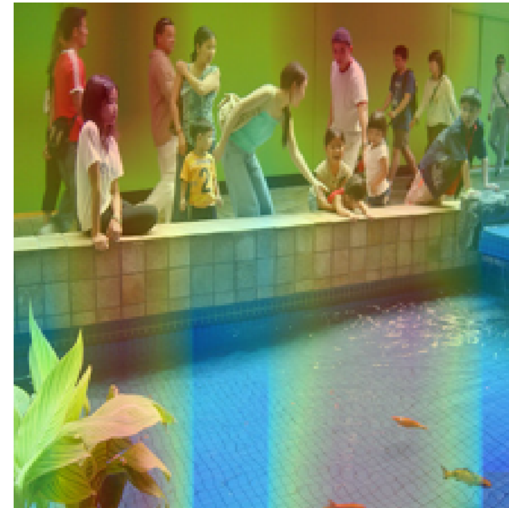
Head 7
