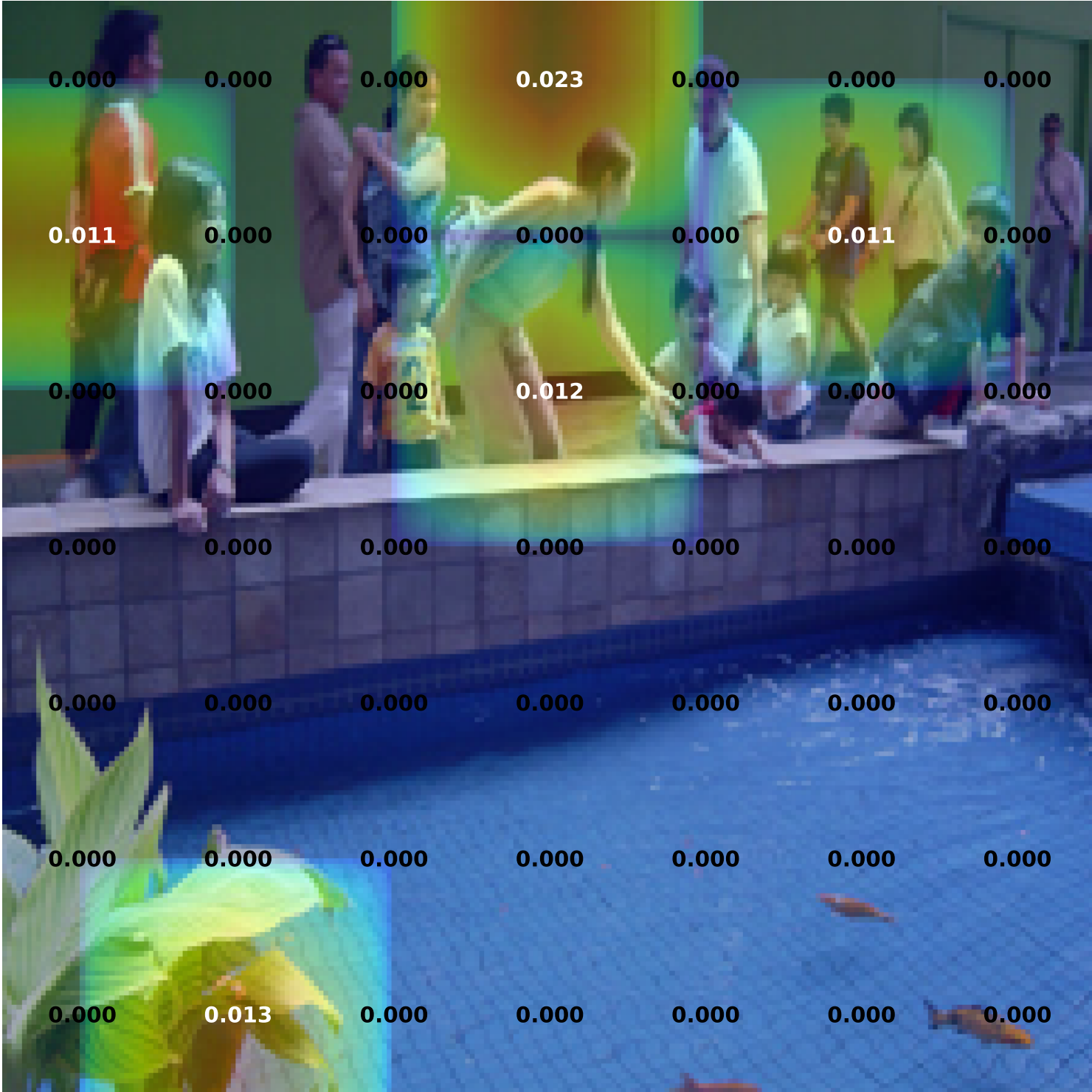
12830823_87d2654e31 Step 3 — RFEM aggregated CLS overlay (values) (K=0.0) \mu = 0.00146 \sigma = 0.004576 (49 patches)
