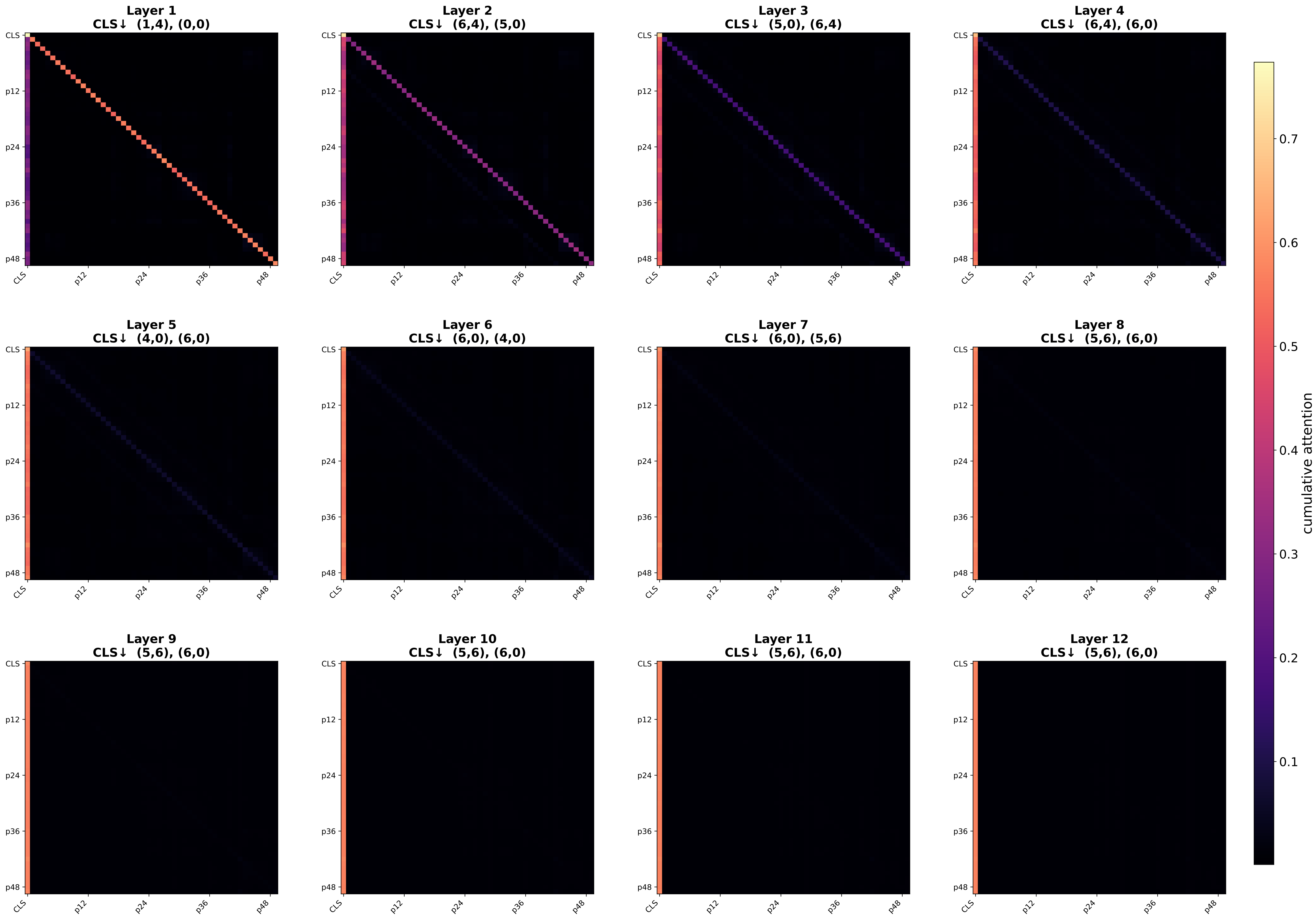
17273391_55cfc7d3d4 — heads-averaged — Cumulative attention rollout matrix per layer (50×50: 1 CLS + 7×7 patches)
