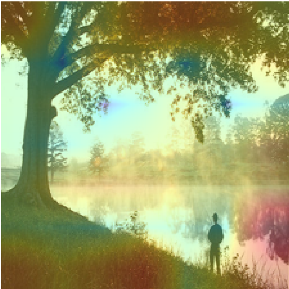
Head 6
