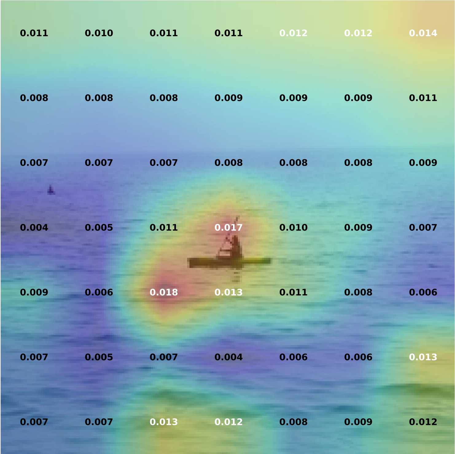
19212715_20476497a3 [vanilla] — Layer 1, Head 1 CLS attention overlay (values) \mu = 0.00911 \sigma = 0.002946 (49 patches)
