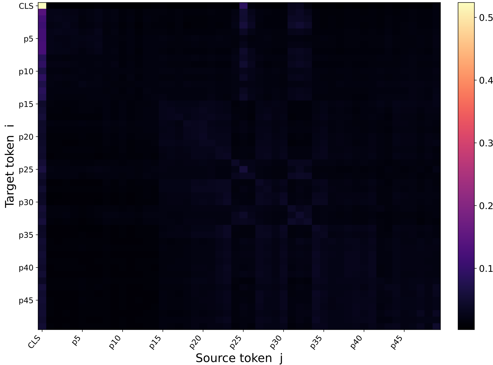
19212715_20476497a3 [vanilla] — Last-layer mean attention matrix \mu = 0.02000 \sigma = 0.014065
