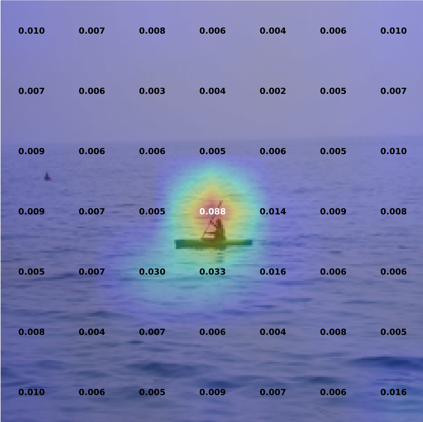
19212715_20476497a3 [vanilla] — Last-layer CLS attention overlay (values) \mu = 0.00972 \sigma = 0.012628 (49 patches)
