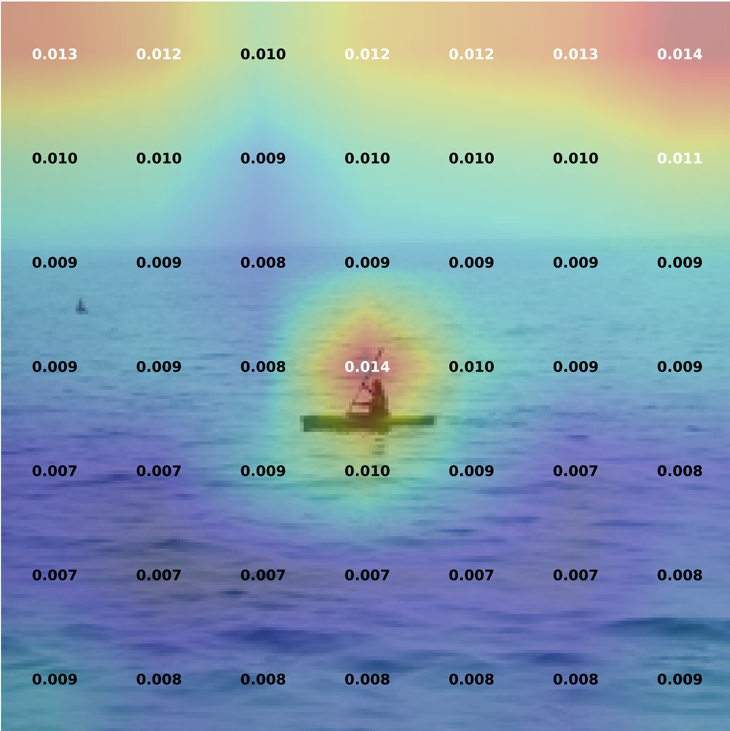
19212715_20476497a3 [rollout] — Standard rollout CLS overlay (values) \mu = 0.00916 \sigma = 0.001794 (49 patches)
