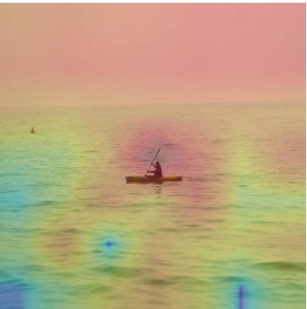
Head 12
