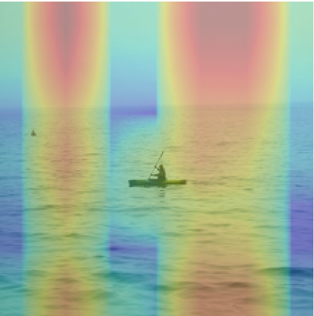
Head 7
