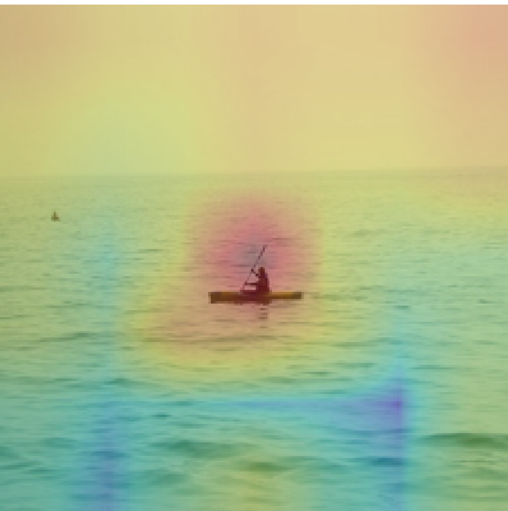
Head 9
