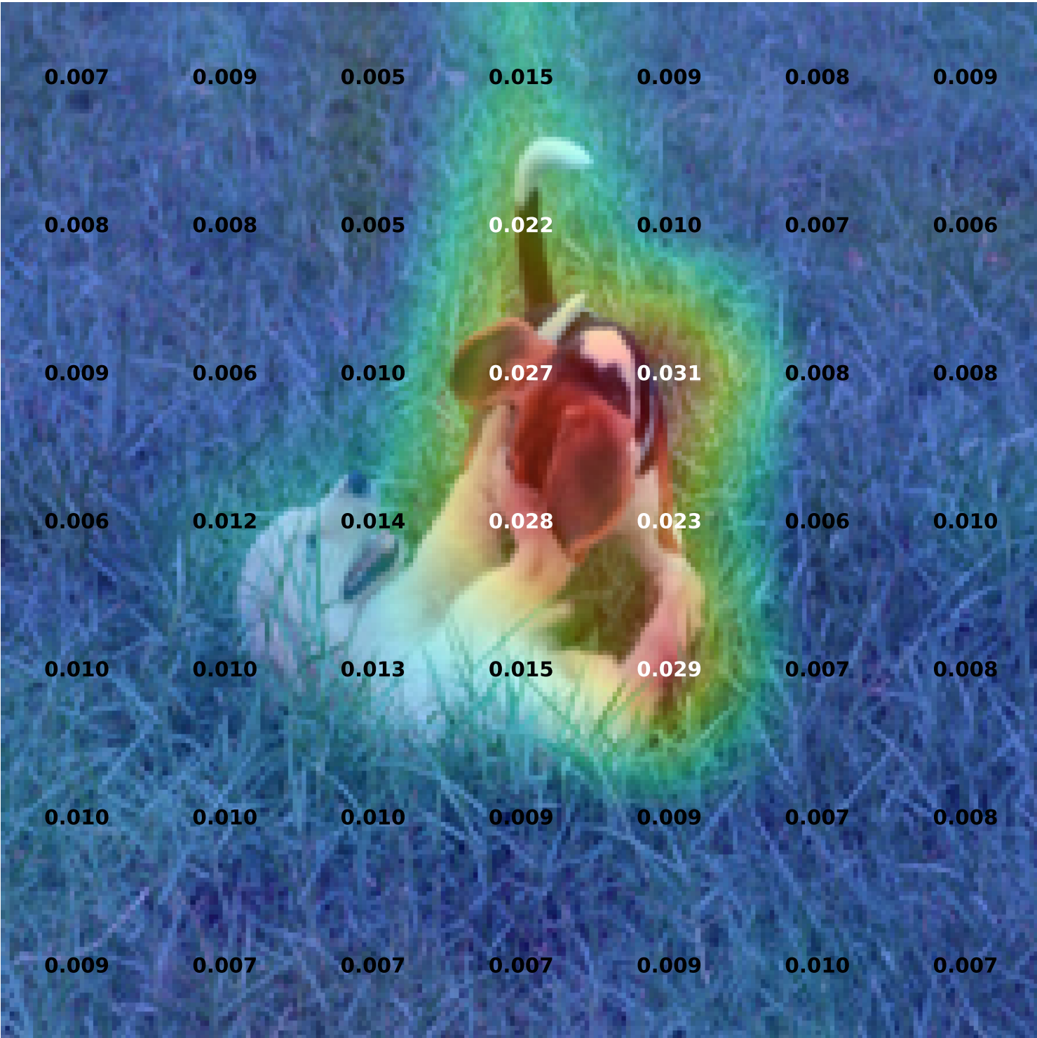
23445819_3a458716c1 [vanilla] — Layer 1, Head 1 CLS attention overlay (values) \mu = 0.01094 \sigma = 0.006374 (49 patches)
