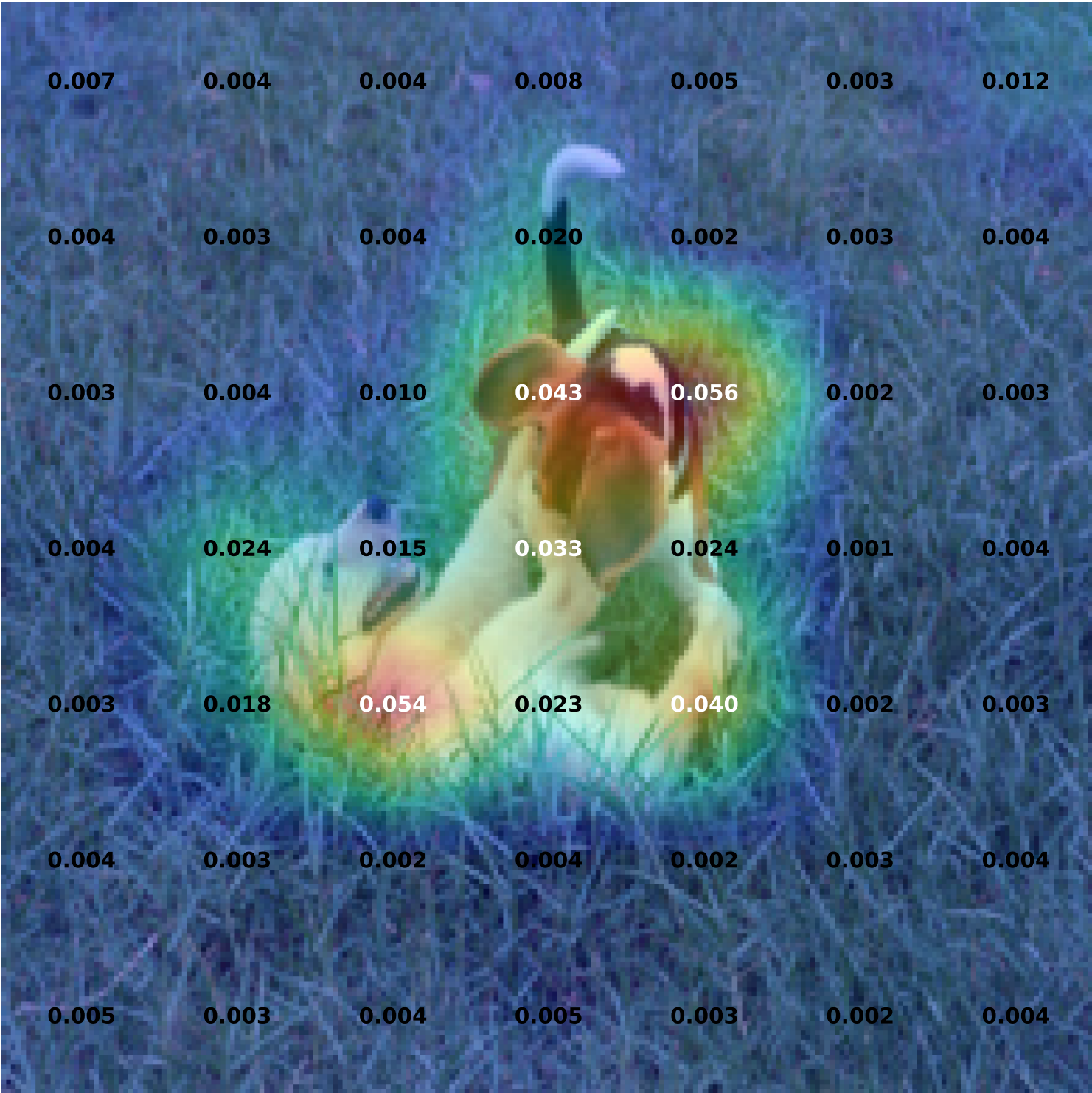
23445819_3a458716c1 [vanilla] — Last-layer CLS attention overlay (values) \mu = 0.01020 \sigma = 0.013434 (49 patches)
