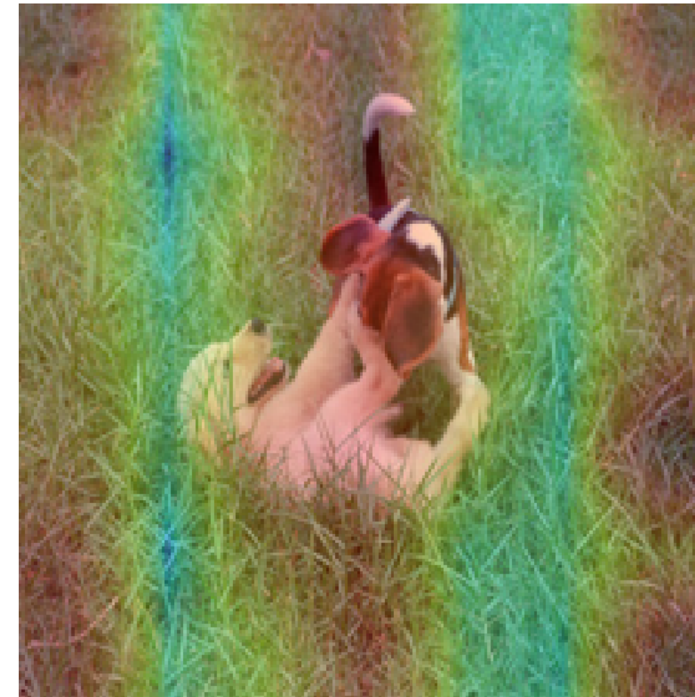
Head 11
