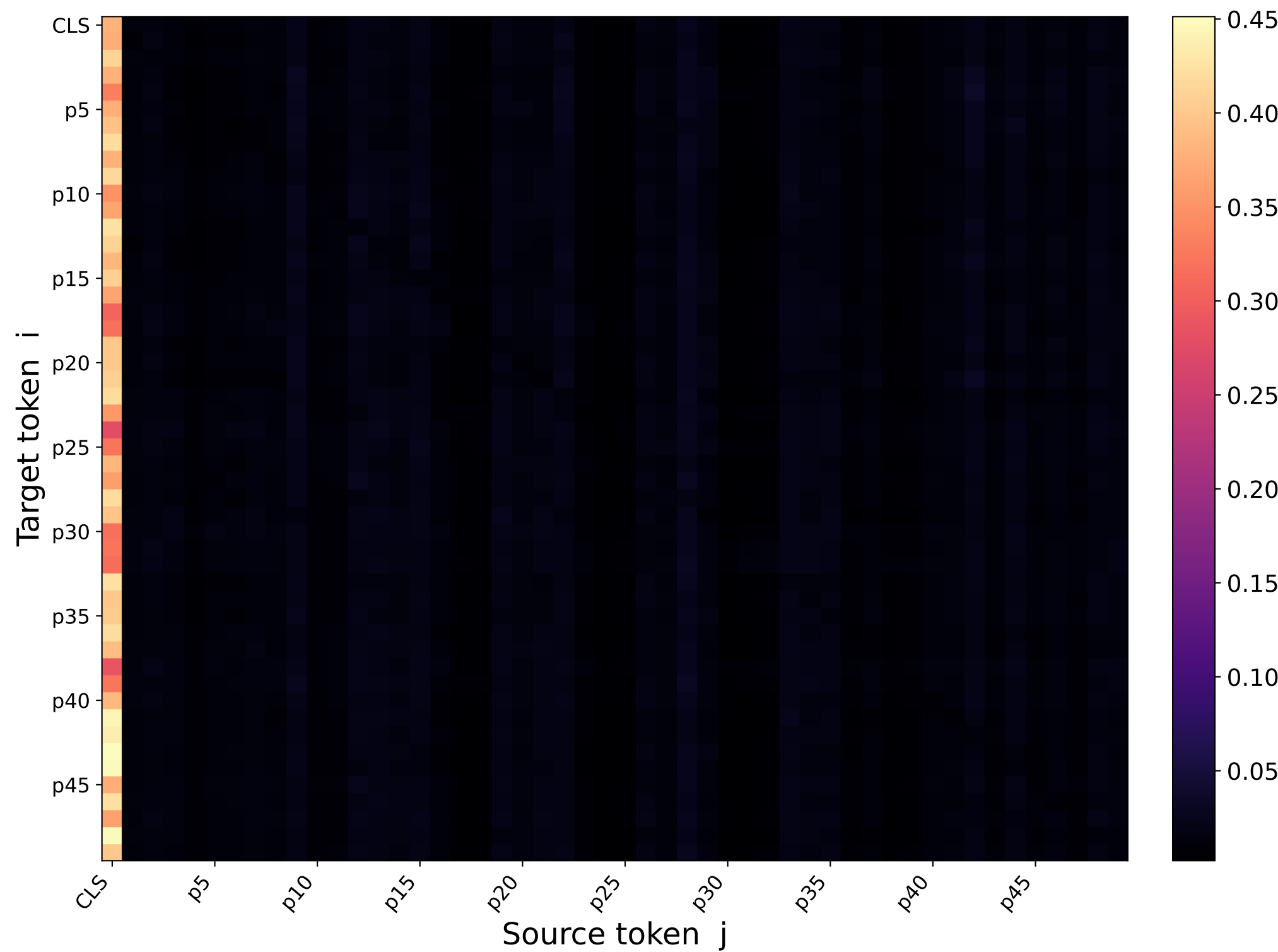
27782020_4dab210360 [vanilla] — Layer 1, Head 1 attention matrix \mu = 0.02000 \sigma = 0.052422
