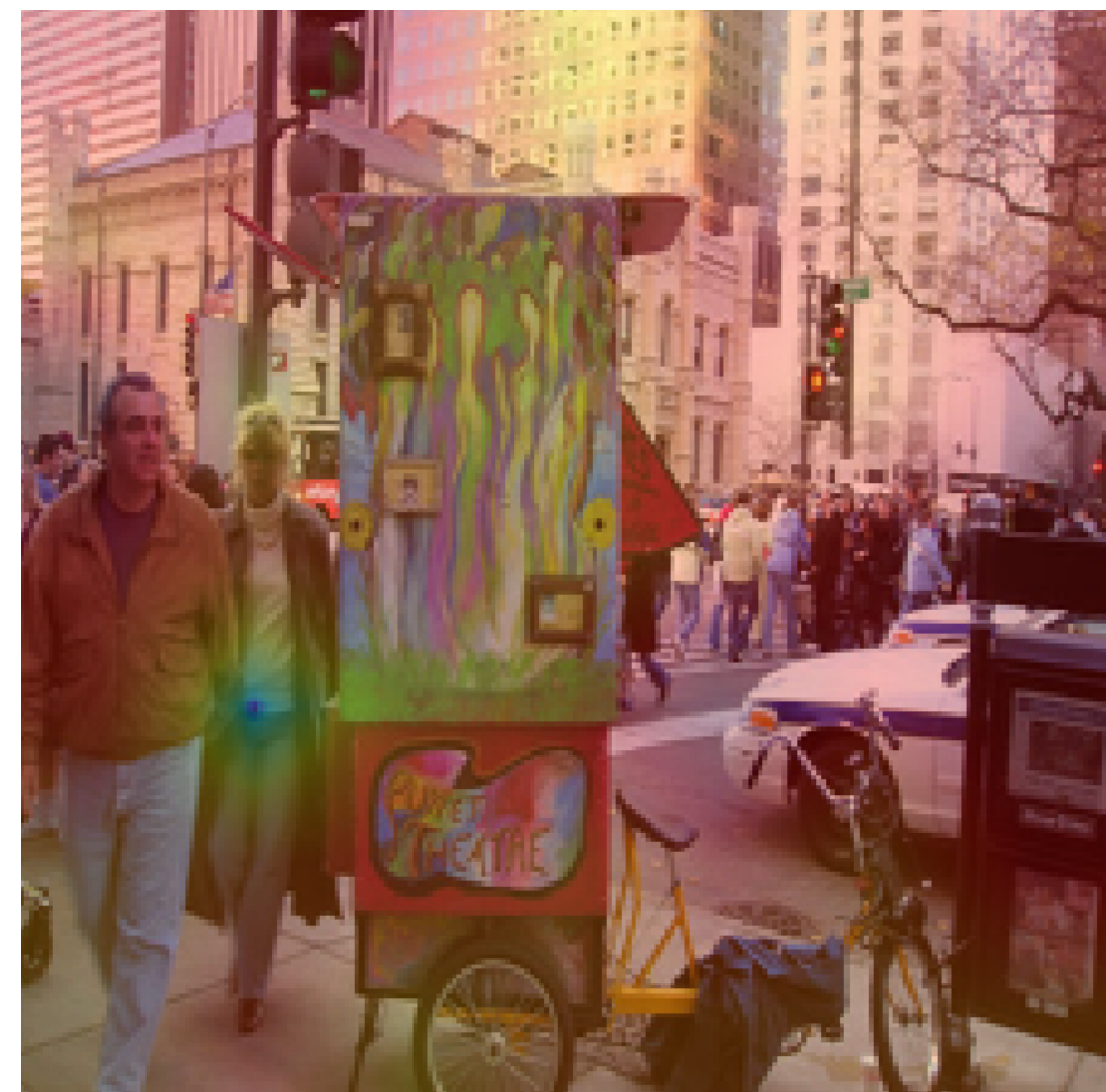
Head 9
