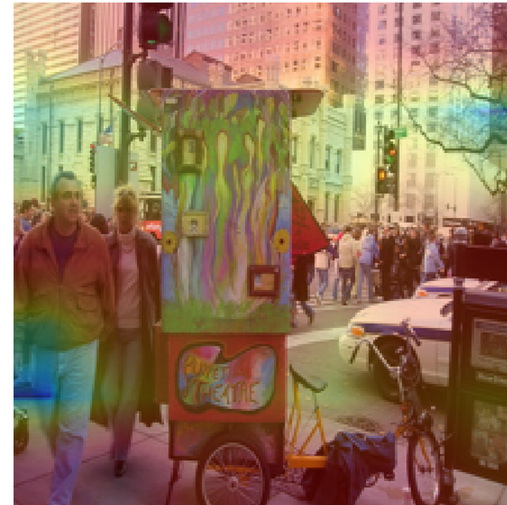
Head 8
