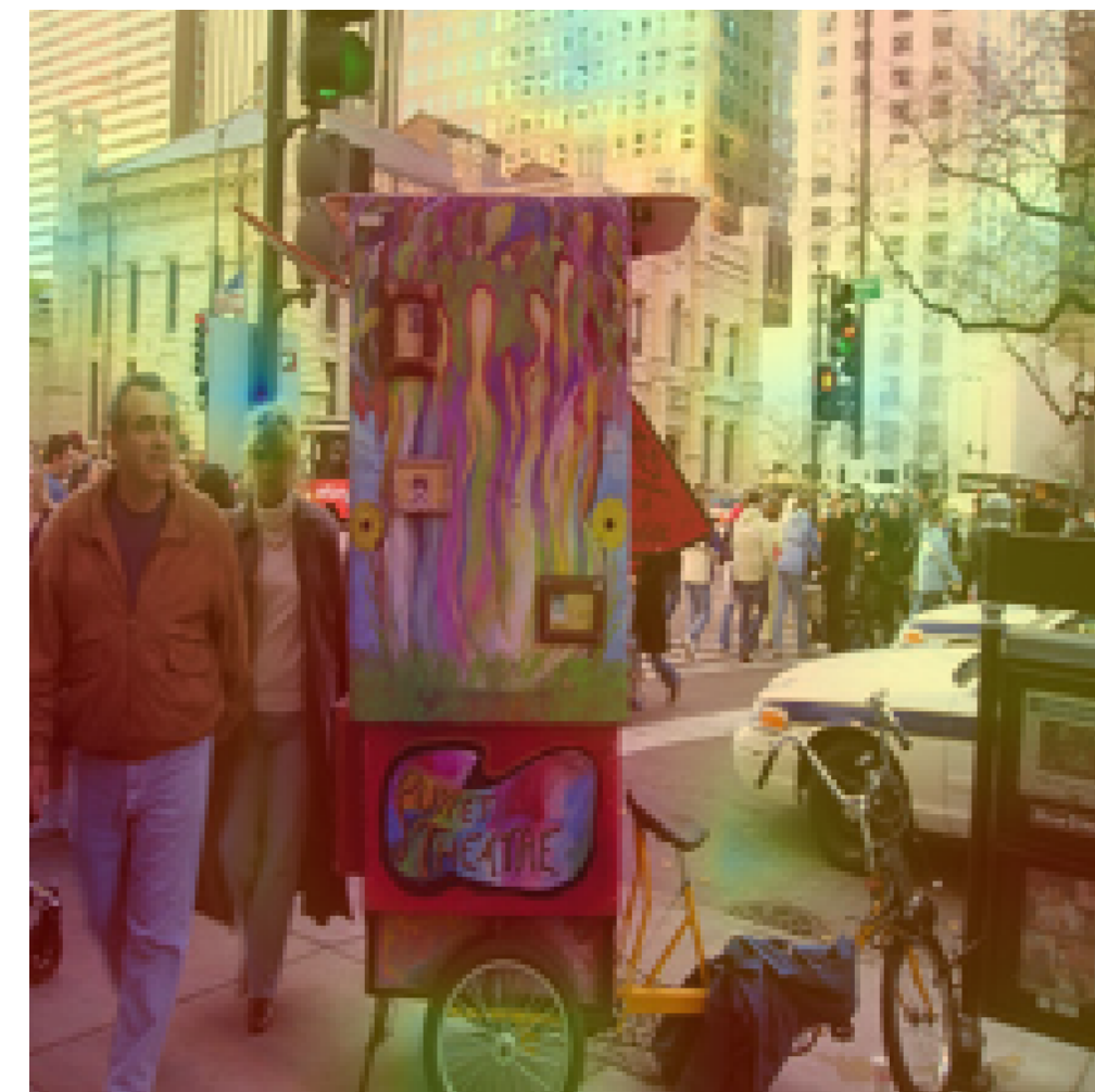
Head 11
