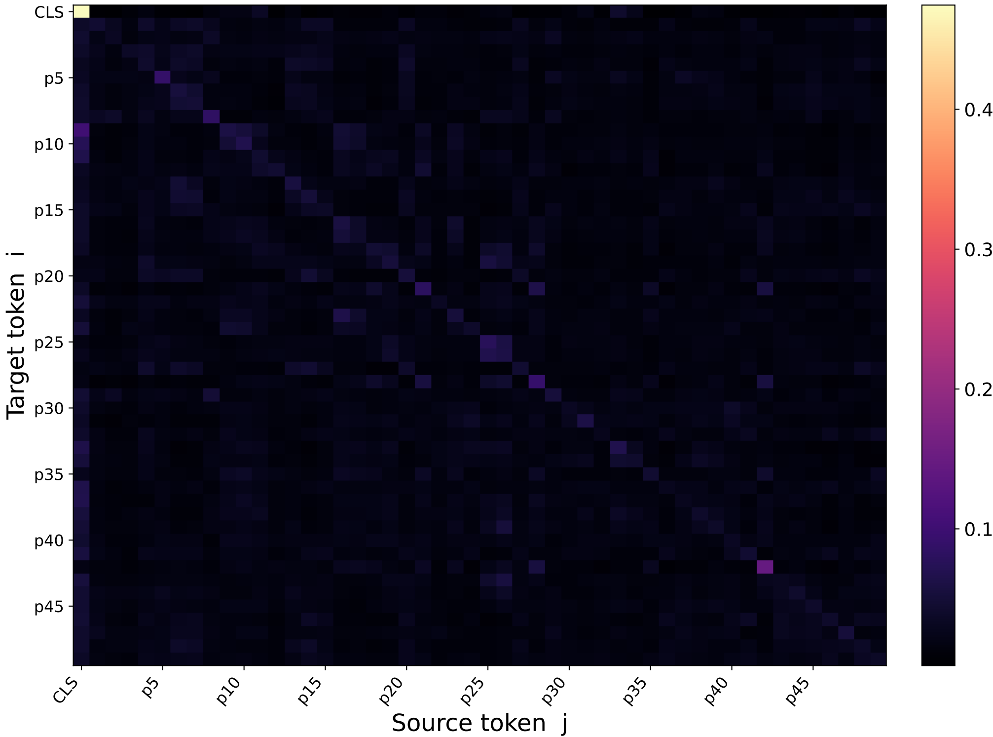
33108590_d685bfe51c [vanilla] — Last-layer mean attention matrix \mu = 0.02000 \sigma = 0.013326
