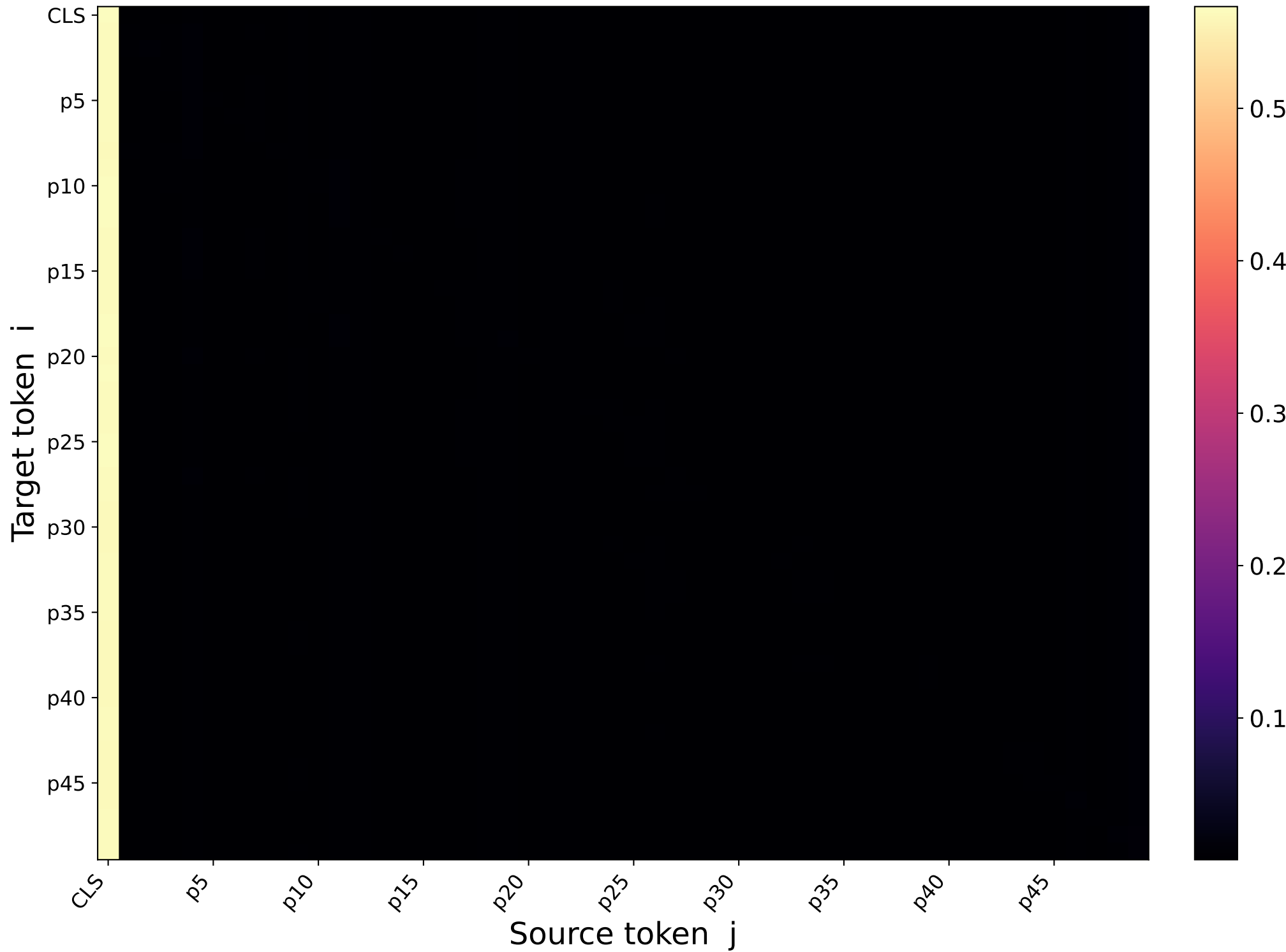
33108590_d685bfe51c [rollout] — Standard attention rollout matrix \mu = 0.02000 \sigma = 0.077617
