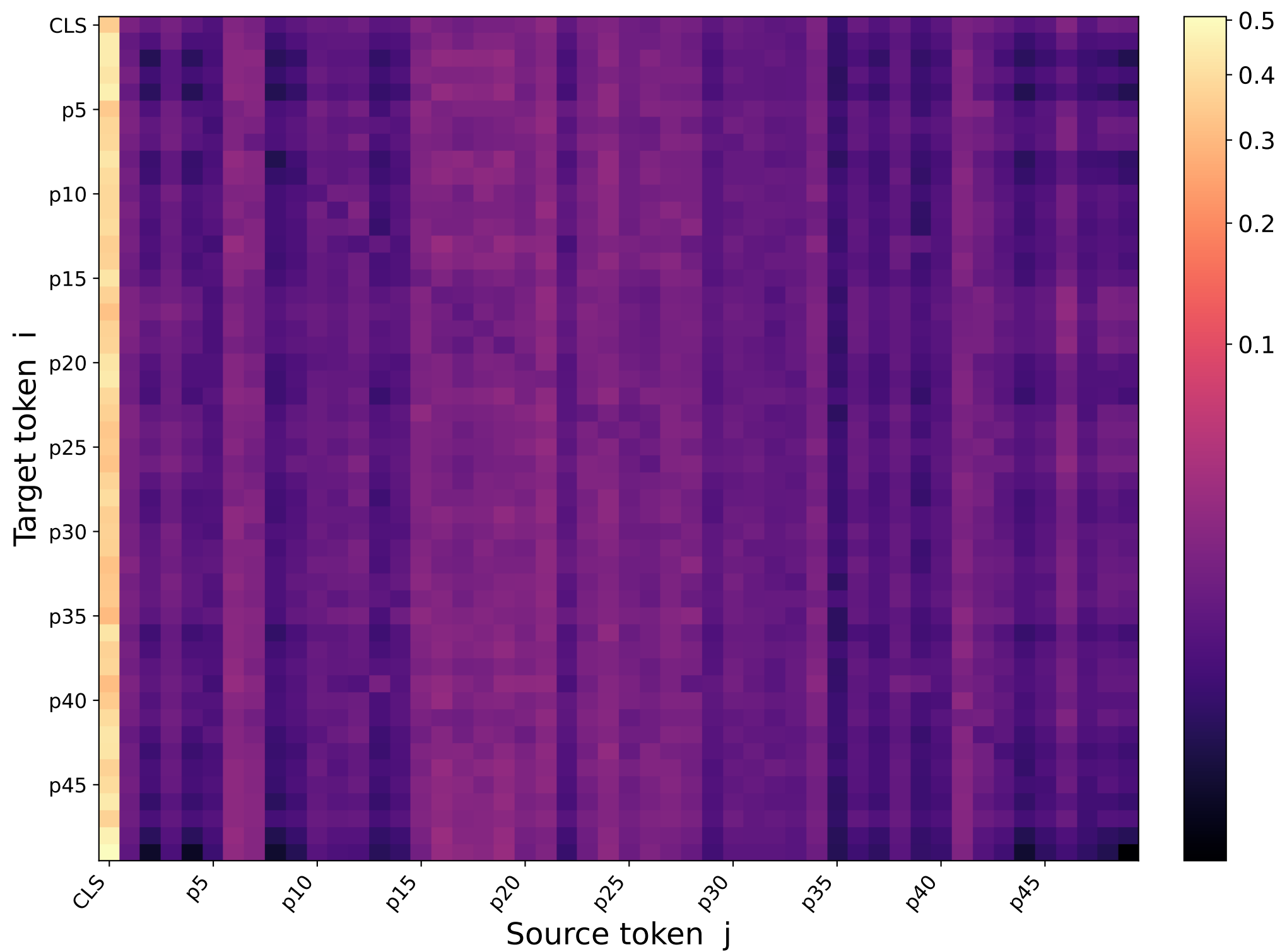
33108590_d685bfe51c Step 1 — Raw attention (Head 1, Layer 1) \mu = 0.02000 \sigma = 0.052793
