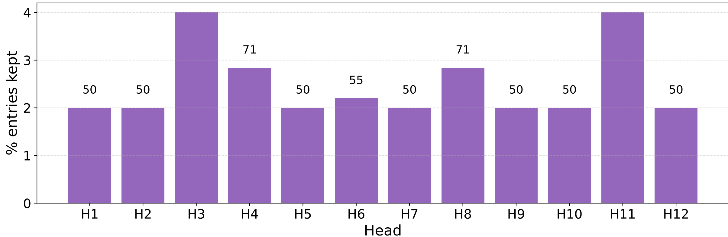
33108590_d685bfe51c Step 2 — Mask sparsity per head (K=0.0)
