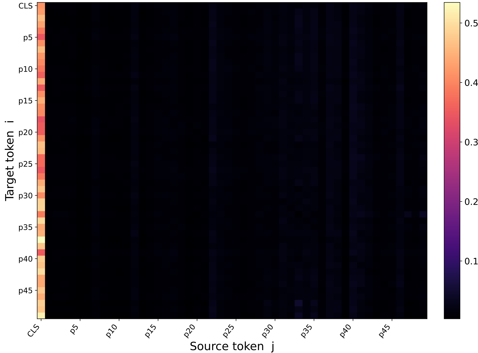
35506150_cbdb630f4f [vanilla] — Layer 1, Head 1 attention matrix \mu = 0.02000 \sigma = 0.058920
