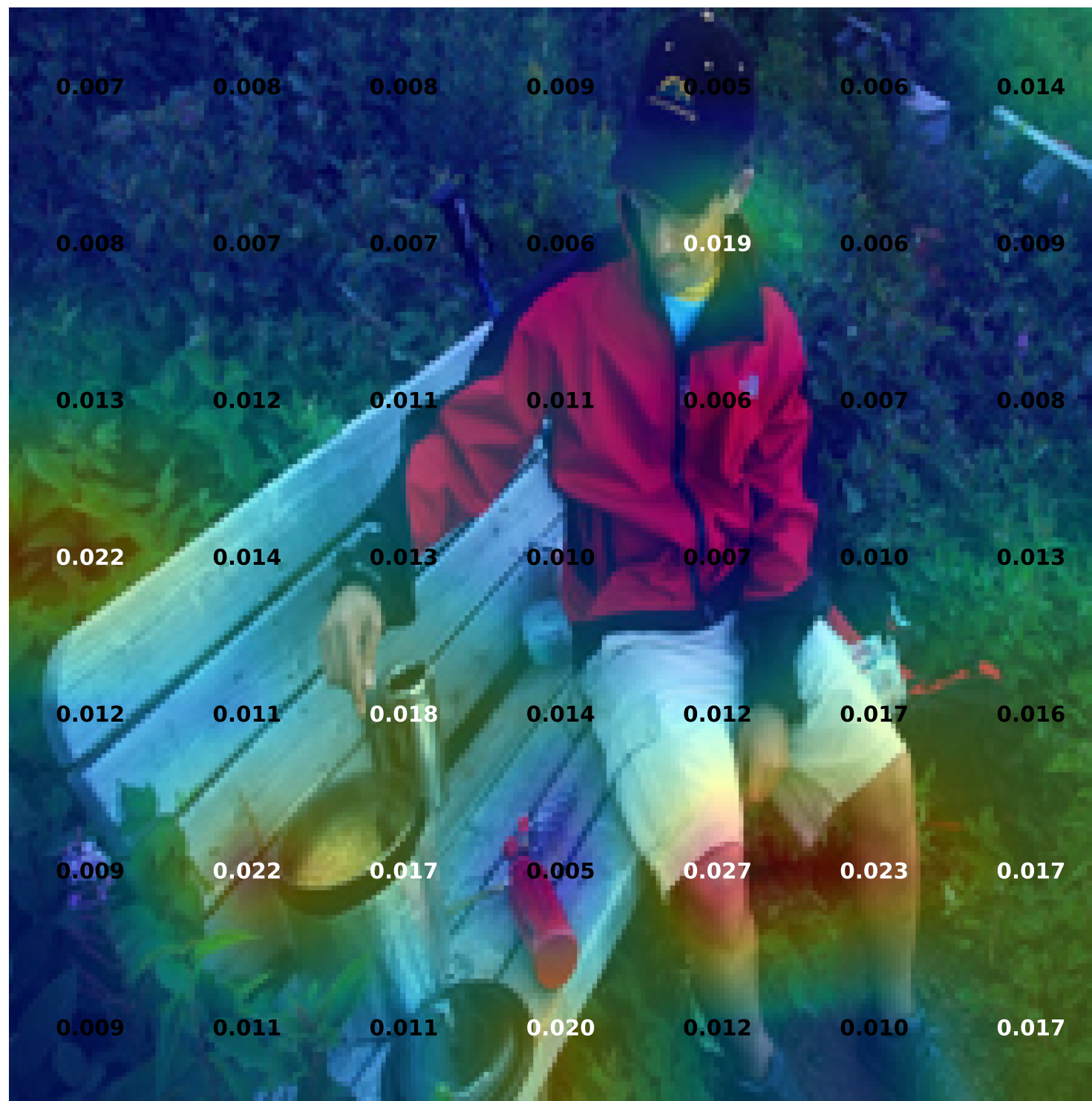
35506150_cbdb630f4f [vanilla] — Layer 1, Head 1 CLS attention overlay (values) \mu = 0.01188 \sigma = 0.005130 (49 patches)
